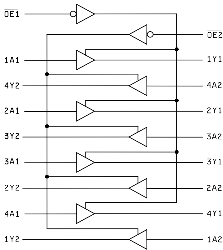
FIGURE 3. Logic diagram.
