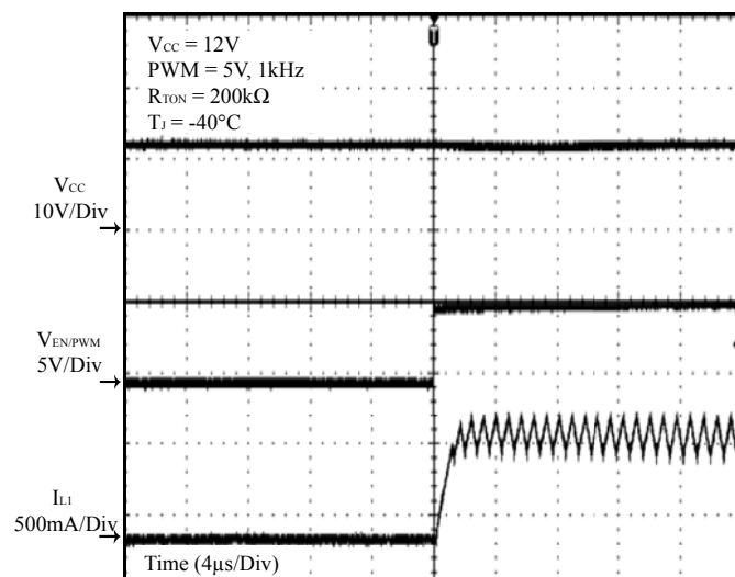
Figure 21 PWM On
