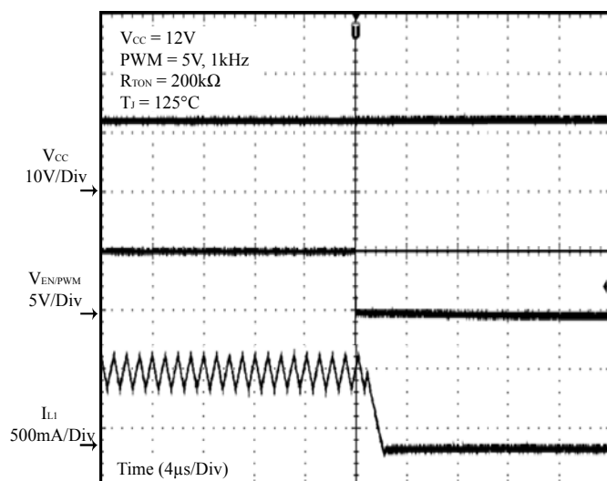
Figure 24 PWM Off
