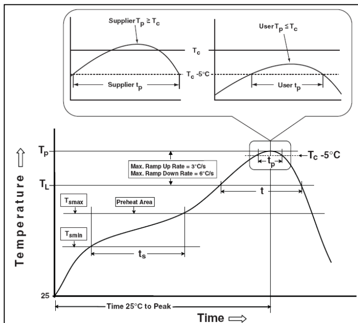
Figure 37 Classification Profile
