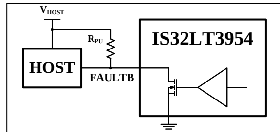
Figure 34 Host Monitors The Fault Reporting
