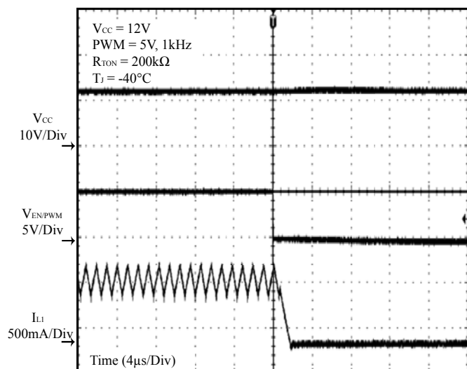
Figure 20 PWM Off
