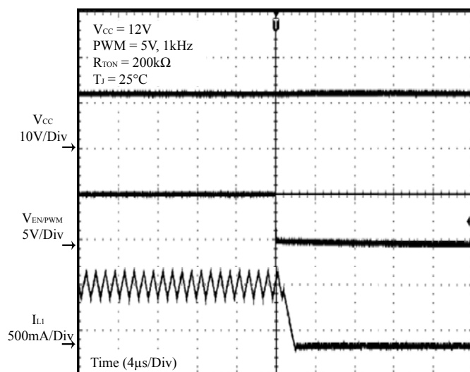
Figure 22 PWM Off
