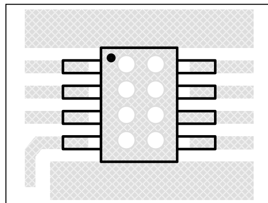
Figure 36 Board Via Layout For Thermal Dissipation
