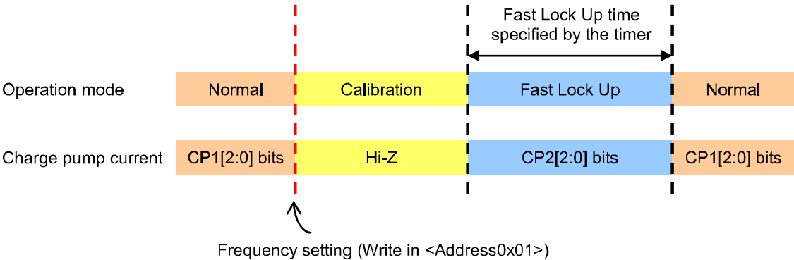
Figure.27 Fast Lock-up Mode Timing Chart
