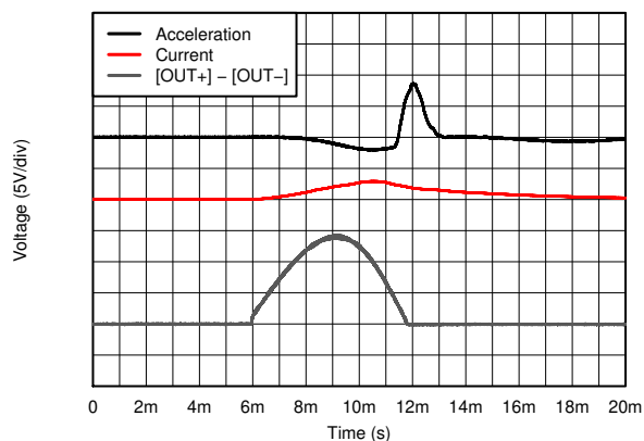
Figure 9. Half Sine Click
