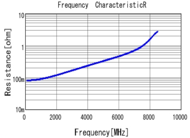
■ GCQ1555C1H7R1CB01 R DC0V, 25degC
