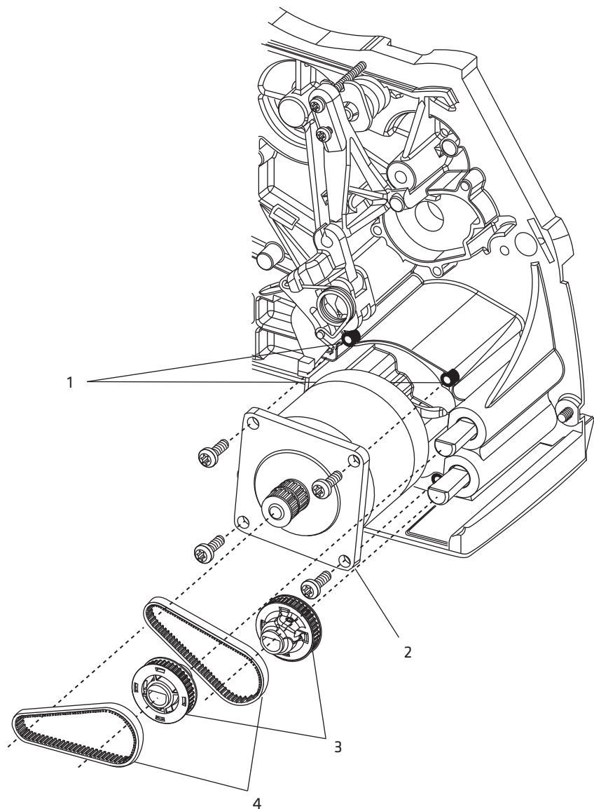
Print Mechanism Electronics Compartment Side 1 Spare Parts
