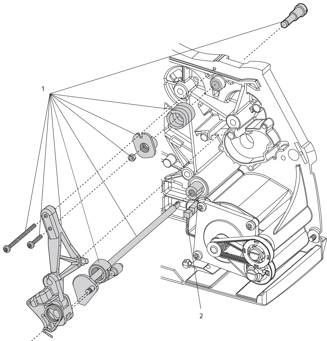
Print Mechanism Electronics Compartment Side 2 Spare Parts
