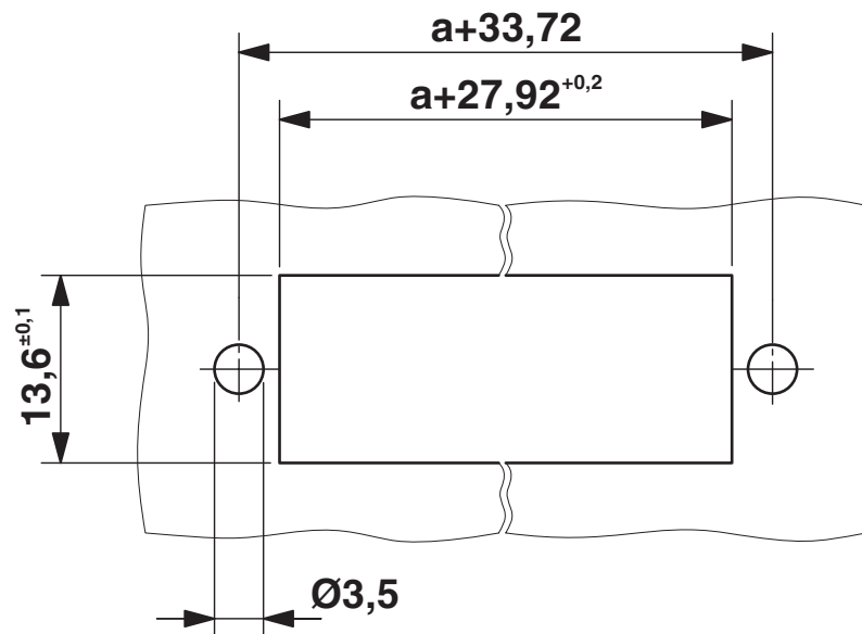
Dimensional drawing
