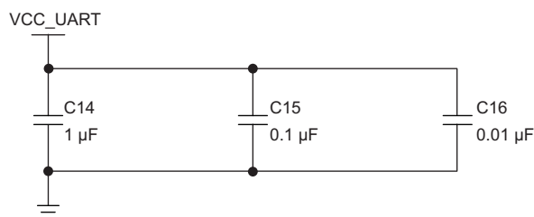
Figure 43. Recommended Bypass Capacitors Array
