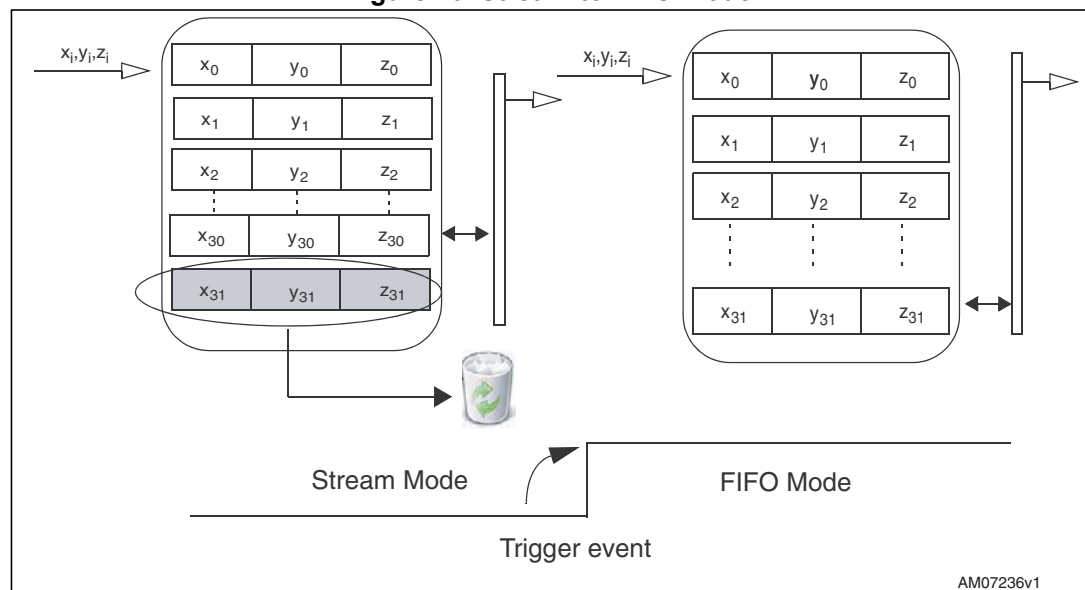
Figure 10. Stream-to-FIFO mode
