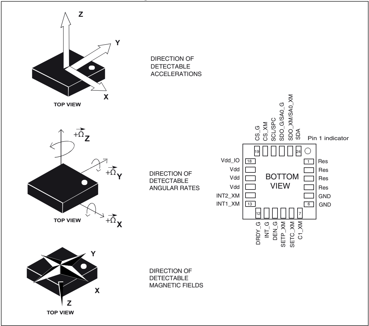
Figure 2. Pin connections
