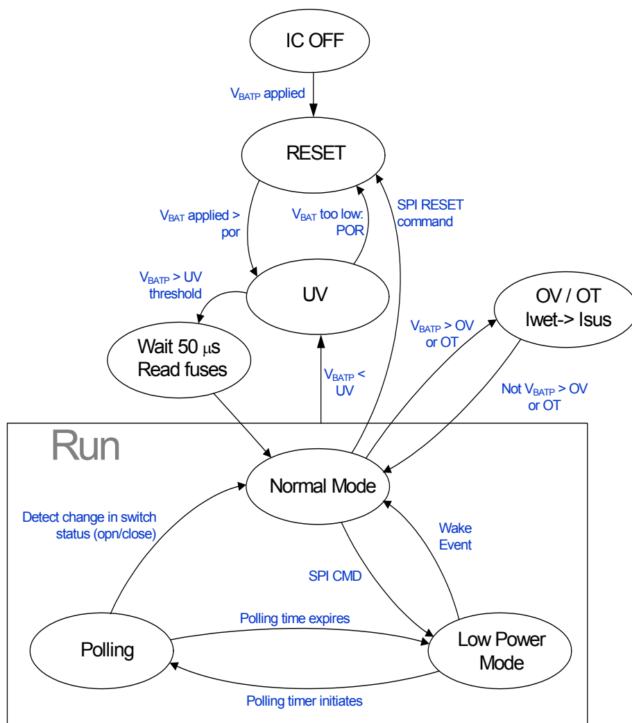
Figure 12. 33978 State Diagram
