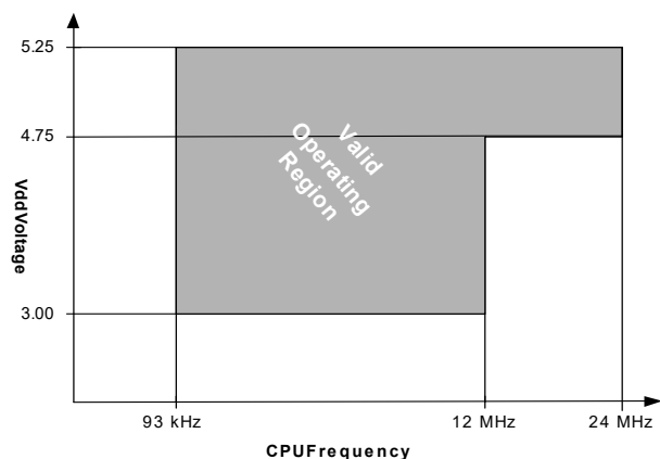
Figure 10. Voltage versus CPU Frequency
