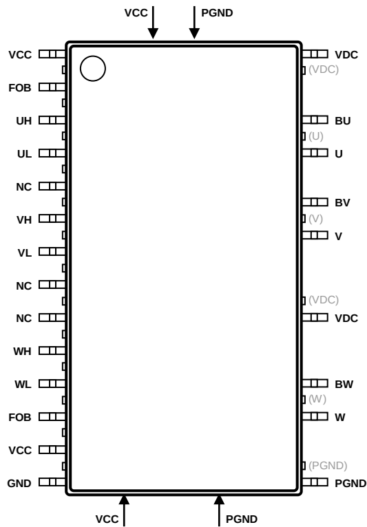
Figure 39. Dummy Pins
