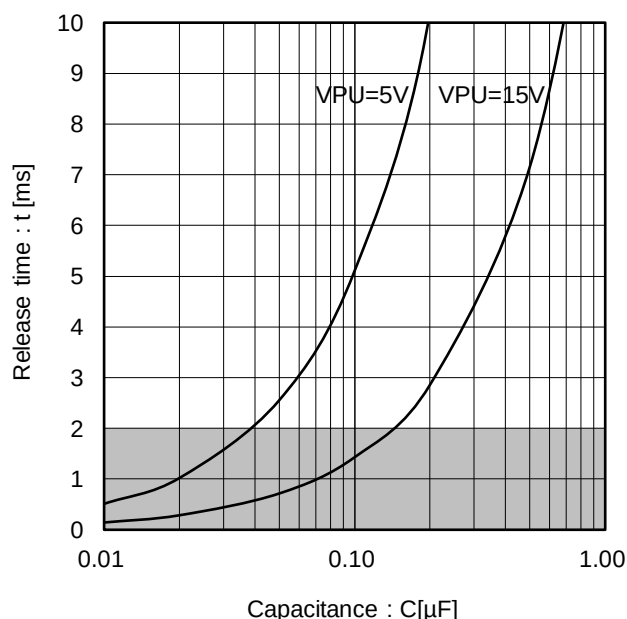
Figure 10. Release Time (Reference Data @R=100kΩ)
