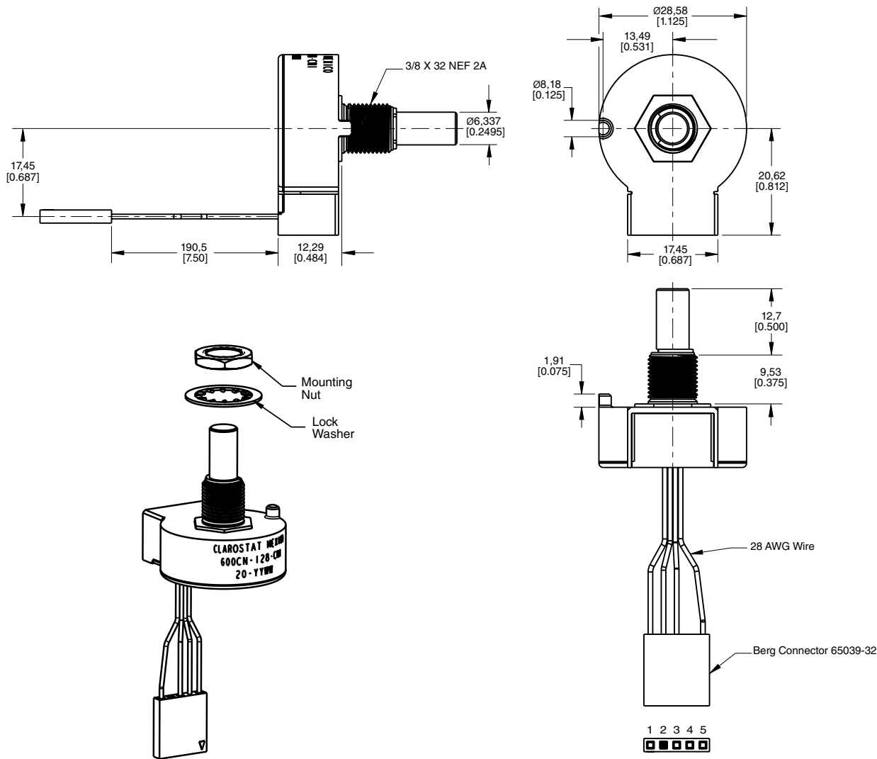
Figure 2. Mounting Hardware
