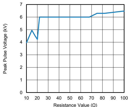
PEAK PULSE VOLTAGE LIMIT FOR AC05-CS: 10 \Omega to 100 \Omega (1.2 / 50 \mu s; 10 pulses at 30 s interval)
