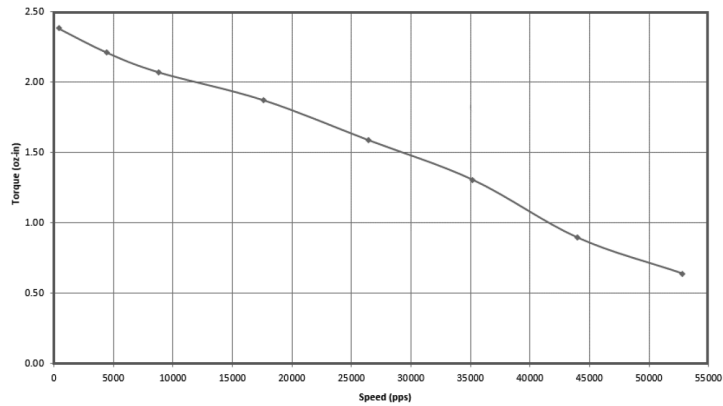
Same Sky P/N NEMA08-13-01D-AMT112S Lin Engineering P/N WD-208-13-01 (1.8 Step Motor) 24 Vdc, 0.60 Amp/Phase, IB462, 1/2 Stepping
