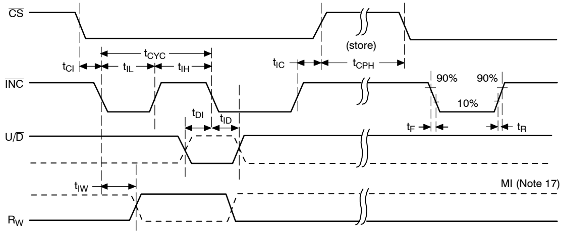
Figure 3. A.C. Timing
