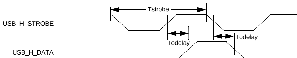
Figure 83. USB HSIC transmit waveform
