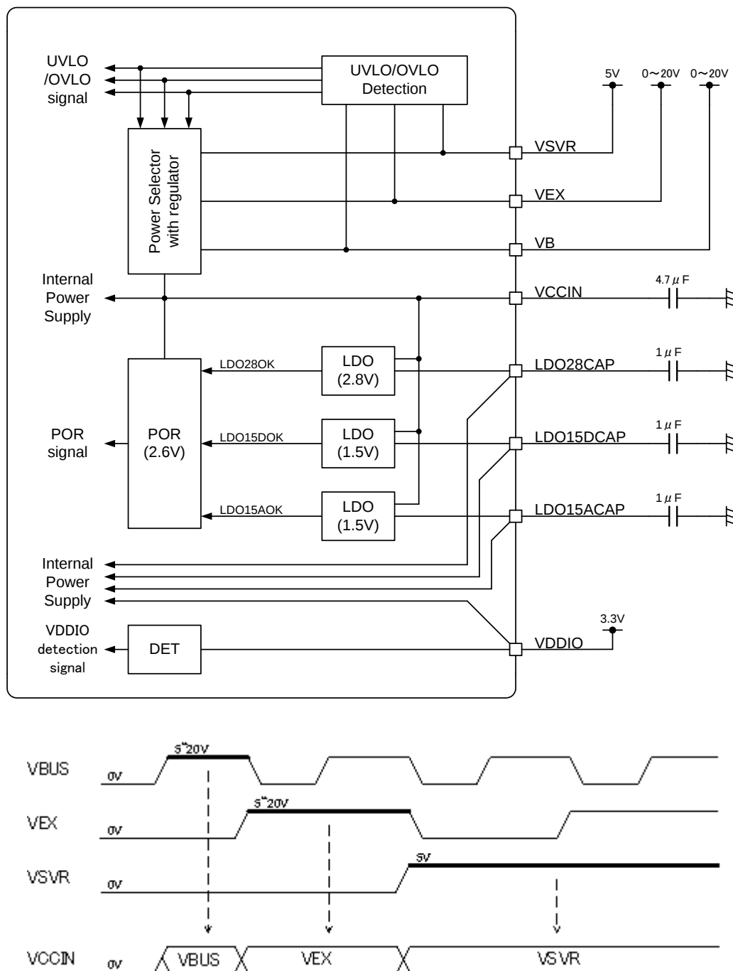
Figure 5-2. Power Supply Management Block Diagram and Timing Chart
