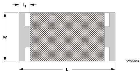
Fig. 5 Chip resistor outlines
