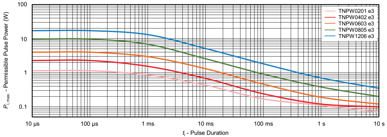
Maximum pulse load, continuous pulse; applicable if \bar{P} \leq P(\vartheta_{amb}) and \hat{U} \leq \hat{U}_{max.} ; for permissible resistance change \pm (0.5 \% R + 0.05 \Omega)
