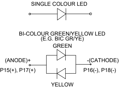
LED SCHEMATIC
