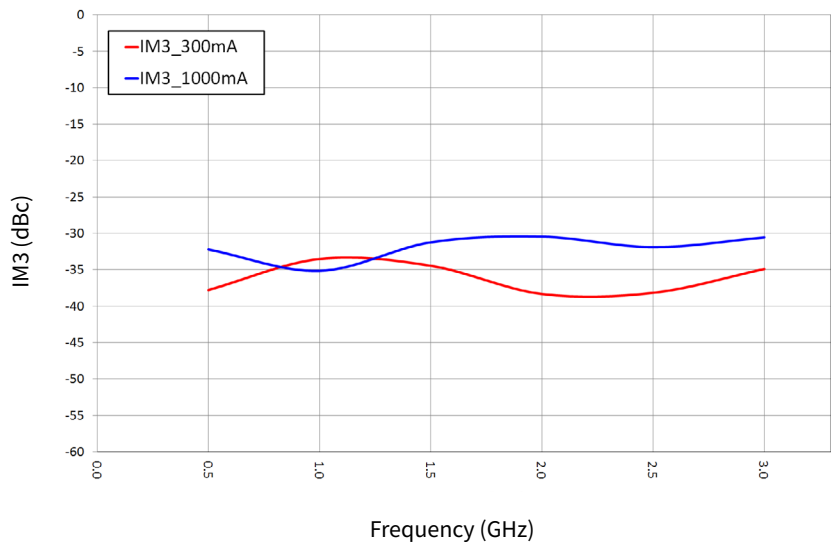
Figure 7. IM3 vs Frequency of the CG2H30070F as Measured in the Single-ended Demonstration Amplifier CG2H30070F-AMP P_{OUT} = 40\text{ dBm} , Temperature = 25 °C
