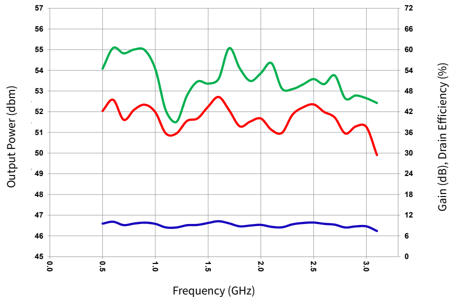
Figure 8. Output Power, Power Gain, and Drain Efficiency vs Frequency of Two CG2H30070F Combined as Measured in the Combined Demonstration Amplifier CG2H30070F-AMP2 with Couplers V_{DD} = 28 \text{ V} , I_{DQ} = 2 \text{ A} , P_{IN} = 42.5 \text{ dBm} , Temperature = 25^\circ \text{C}
