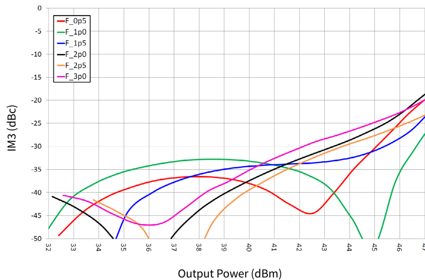
Figure 5. IM3 vs Output Power of the CG2H30070F as Measured in the Single-ended Demonstration Amplifier CG2H30070F-AMP I_{DQ} = 300 \text{ mA} , Temperature = 25 °C
