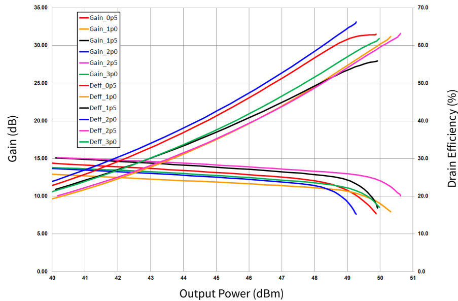
Figure 3. Gain and Drain Efficiency vs Output Power at Various Frequencies as Measured in the Single-ended Demonstration Amplifier CG2H30070F-AMP CW-Operation, V_{DD} = 28\text{ V} , I_{DQ} = 1.0\text{ A}
