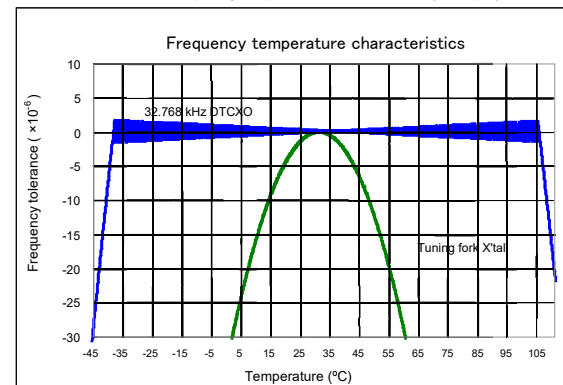
■ 32.768 kHz-DTCXO Frequency temperature characteristics (Example)
