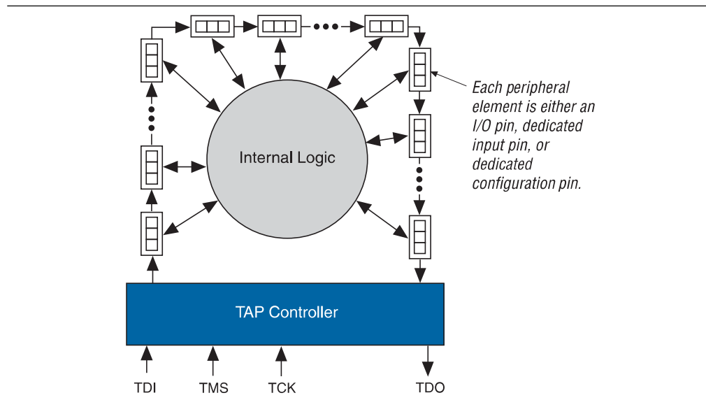
Figure 8-3. Boundary-Scan Register
