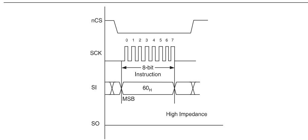
Figure 7-27. UFM-ERASE Operation Sequence
