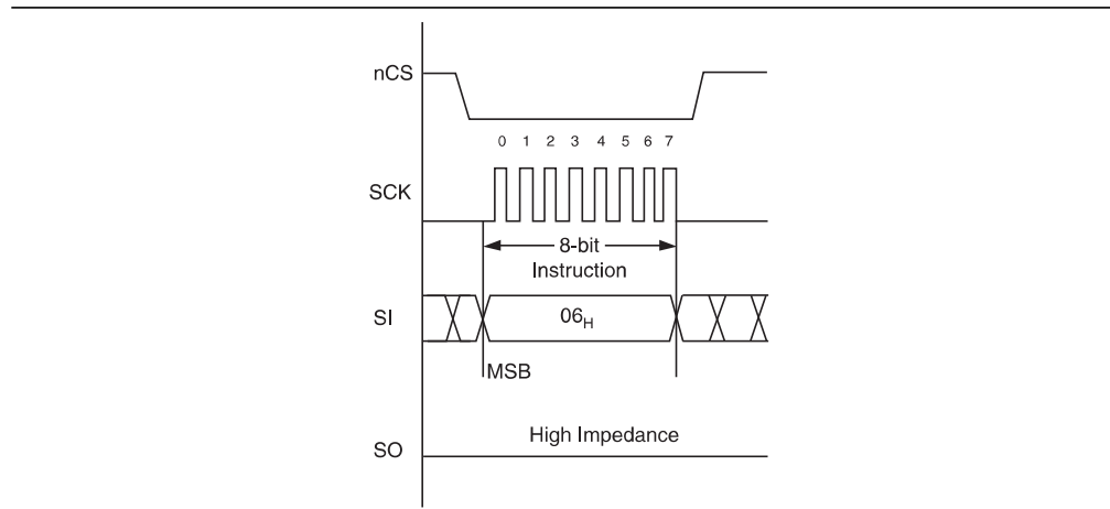
Figure 7-28. WREN Operation Sequence
