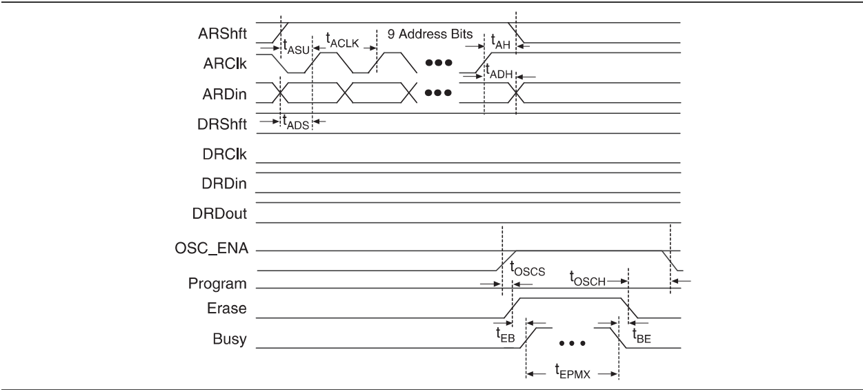
Figure 3-5. UFM Erase Waveform
