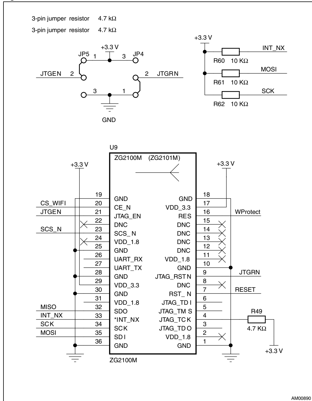
Figure 23. Wi-Fi module-2
