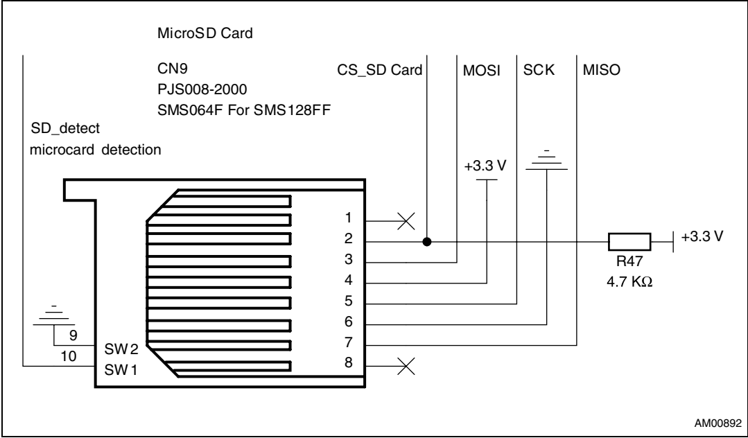
Figure 24. MicroSD Card
