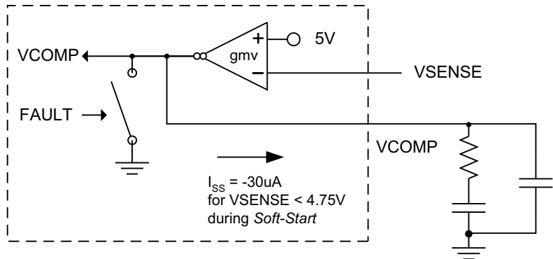
Figure 20. Soft Start
