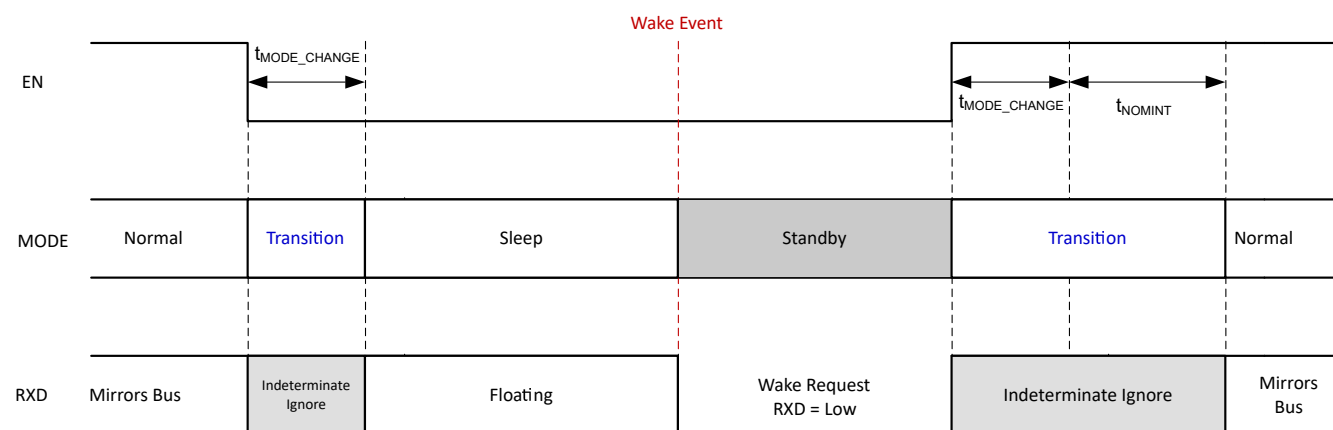
Figure 8-15. Mode Transitions
