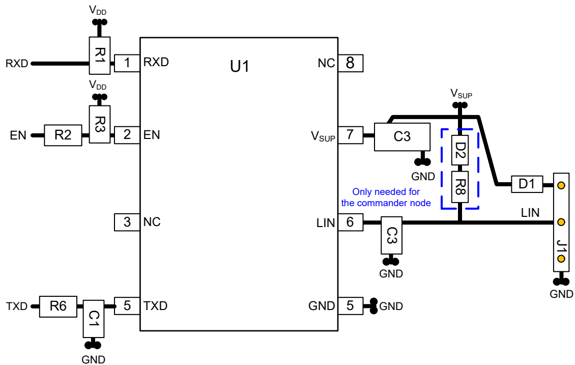
Figure 12-1. Layout Example
