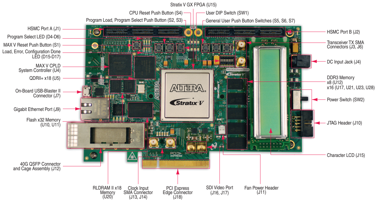
Figure 2-1. Overview of the Stratix V GX FPGA Development Board Features
