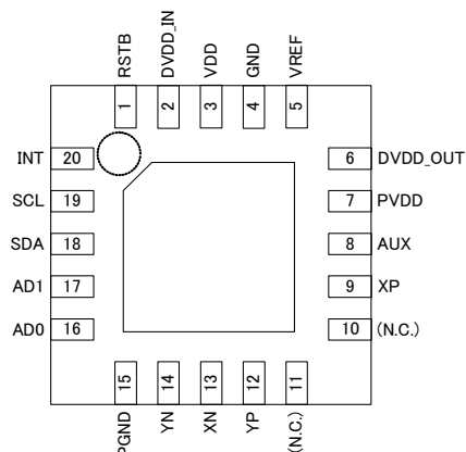
BOTTOM VIEW (LEAD SIDE UP)
