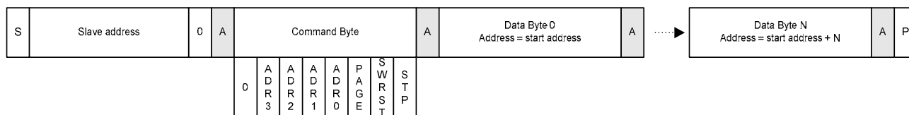
Figure 1. Write Protocol
