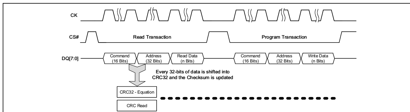
Figure 38 CRC calculation overview
