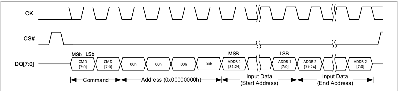
Figure 22 Octal SDR transaction with command and two input addresses
