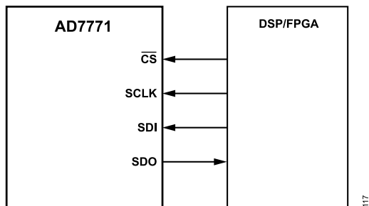
Figure 117. SPI Control Interface—AD7771 is the SPI Subordinate, Digital Signal Processor (DSP)/Field Programmable Gate Array (FPGA) is the Main
