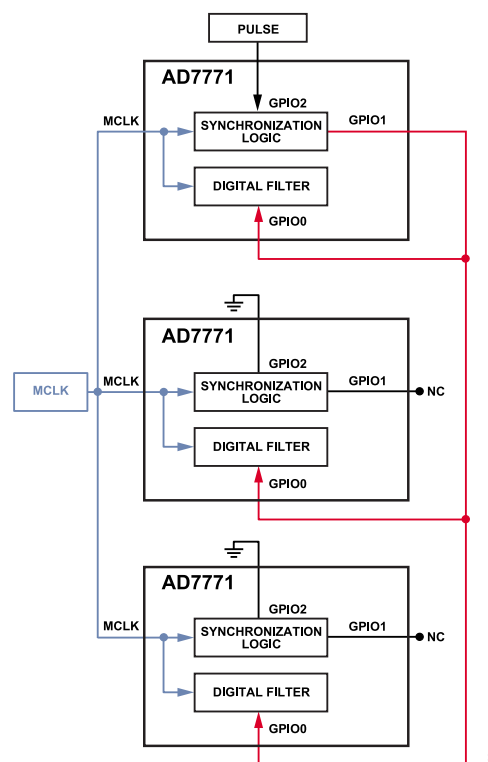
Figure 126. Hardware ODR Update
