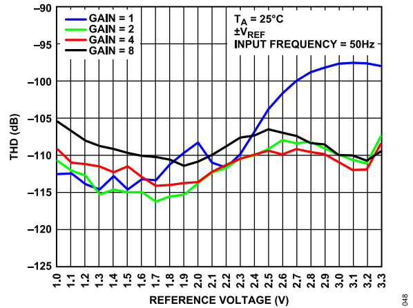
Figure 48. THD vs. Reference Voltage at 16 kSPS, Low Power Mode
