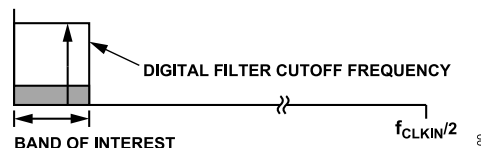
Figure 100. \Sigma - \Delta ADC Operation, Removal of Noise Energy from the Band of Interest (Linear Scale X-Axis)
