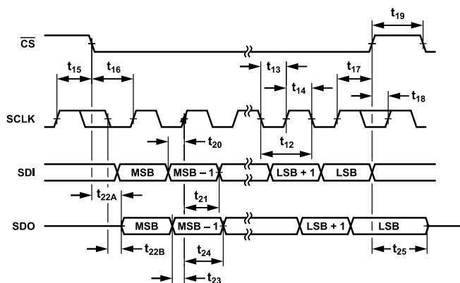
Figure 3. SPI Control Interface Timing Diagram
