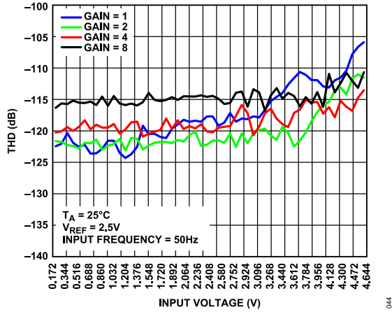
Figure 44. THD vs. Input Voltage at 64 kSPS, High Resolution Mode
