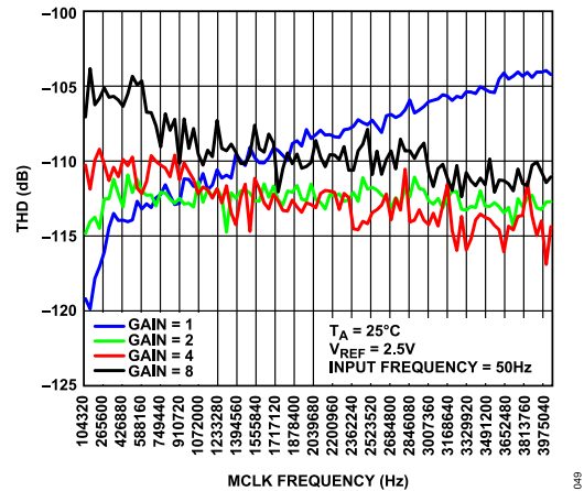
Figure 49. THD vs. Main Clock Frequency, Low Power Mode
