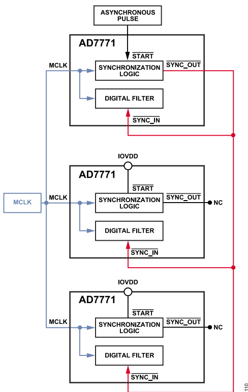
Figure 110. Multiple AD7771 Devices Synchronization
