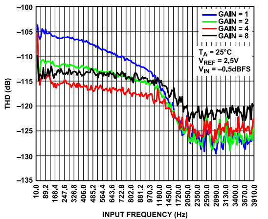
Figure 40. THD vs. Input Frequency at 16 kSPS, High Resolution Mode, Sinc3 Filter Enabled
