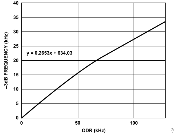
Figure 129. -3 dB Correction Factor, Sinc3 Filter Enabled
