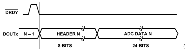
Figure 124. ADC Output—8-Bit Header Plus 24-Bit Conversion Data
