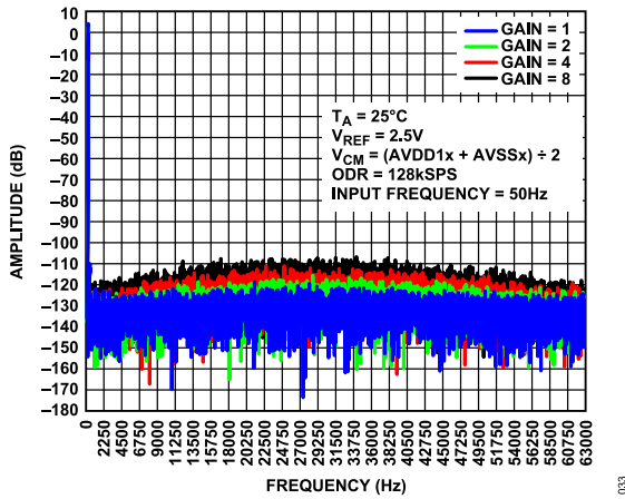
Figure 33. FFT Plot, High Resolution Mode at 128 kSPS, Input Frequency ( f_{IN} ) = 50 Hz, Sinc5 Filter Enabled
