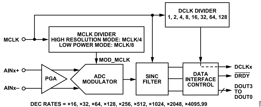
Figure 109. Clock Generation on the AD7771
