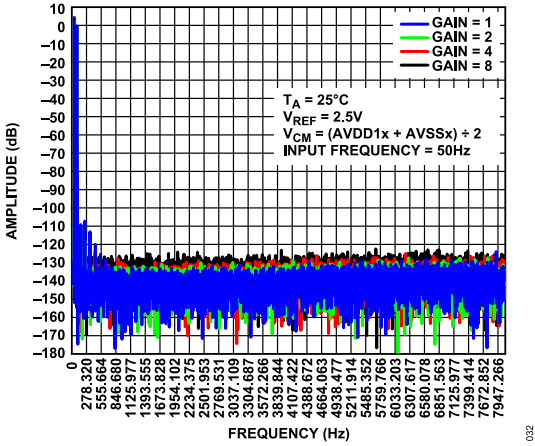
Figure 32. FFT Plot, High Resolution Mode at 16 kSPS, Input Frequency ( f_{IN} ) = 50 Hz, Sinc3 Filter Enabled
