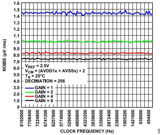
Figure 26. Noise vs. Clock Frequency, High Resolution Mode
