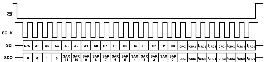
Figure 120. SAR ADC/Diagnostic Mode—CRC Enabled
