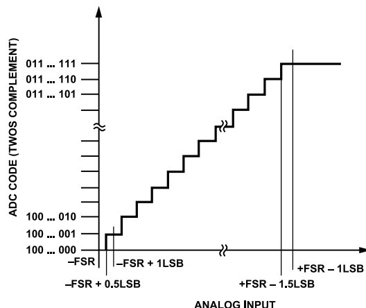
Figure 106. Transfer Function
