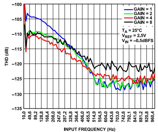
Figure 43. THD vs. Input Frequency at 4 kSPS, Low Power Mode, Sinc3 Filter Enabled
