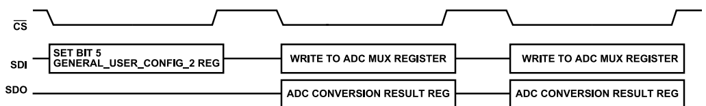
Figure 121. SPI Used to Read Back the Σ-Δ ADC Data, in 24-Bit Frames
