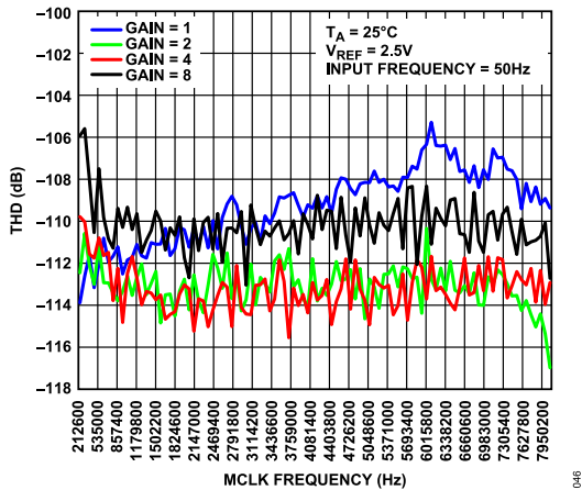
Figure 46. THD vs. Main Clock Frequency, High Resolution Mode
