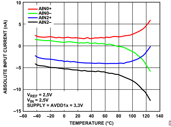
Figure 74. Absolute Input Current vs. Temperature, High Resolution Mode
