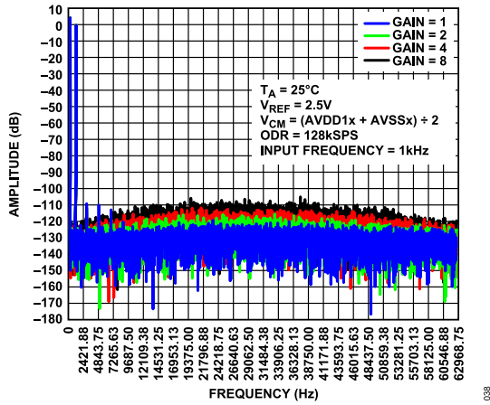
Figure 38. FFT Plot, High Resolution Mode at 128 kSPS, Input Frequency ( f_{IN} ) = 1 kHz, Sinc5 Filter Enabled
