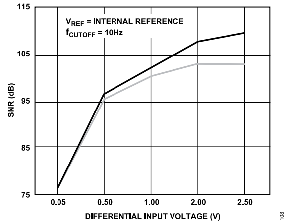
Figure 108. SNR Adding External LPF with V_{REF} = Internal Reference and f_{CUTOFF} = 10 Hz
