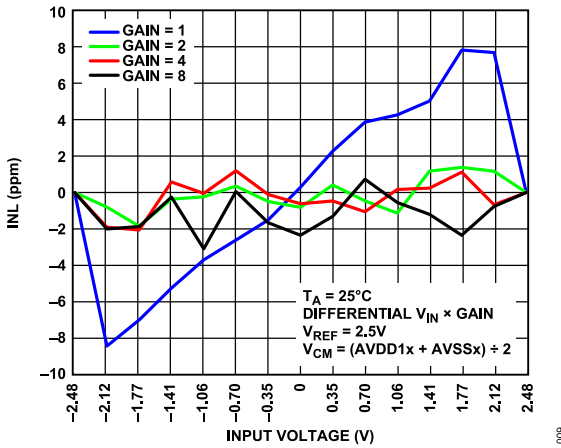
Figure 9. INL vs. Input Voltage and PGA Gain at 64 kSPS, High Resolution Mode
