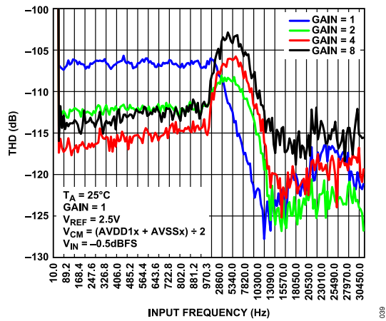
Figure 39. THD vs. Input Frequency at 64 kSPS, High Resolution Mode, Sinc5 Filter Enabled
