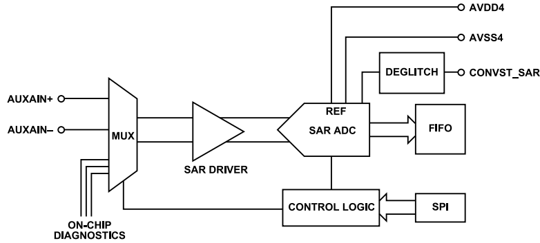
Figure 123. SAR ADC Configuration and Control
