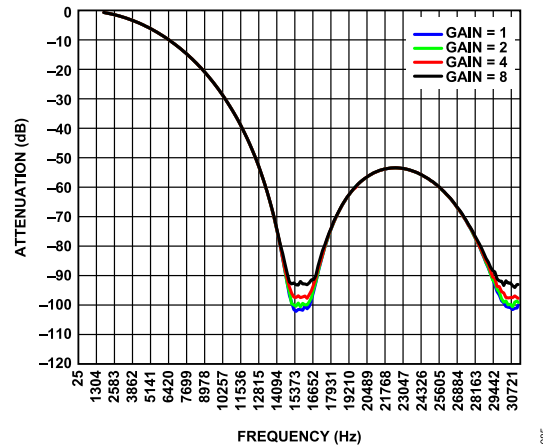
Figure 85. Filter Profiles at 16 kSPS, Low Power Mode
