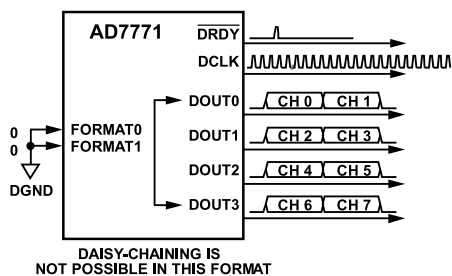
Figure 131. FORMATx Pin Configuration—FORMAT0 = 0, FORMAT1 = 0
