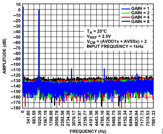
Figure 34. FFT Plot, High Resolution Mode at 16 kSPS, Input Frequency ( f_{IN} ) = 1 kHz, Sinc3 Filter Enabled
