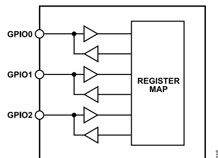
Figure 116. GPIOx Pin Functionality
