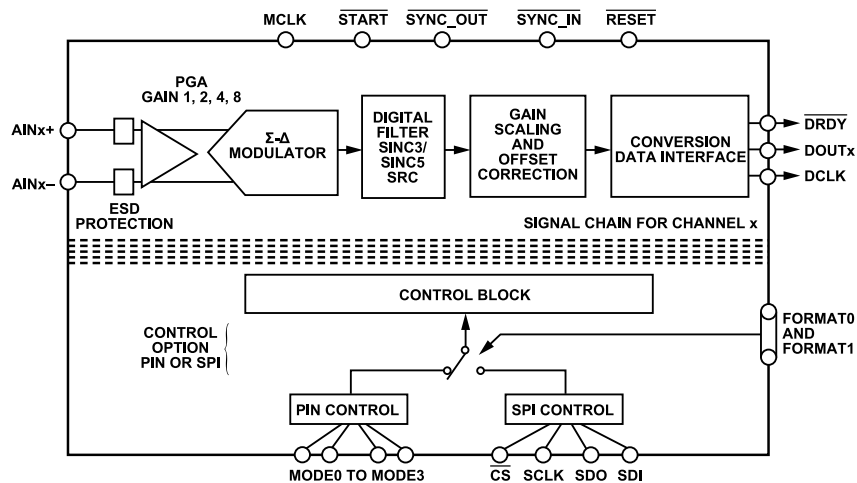
Figure 107. Top Level Core Signal Chain
