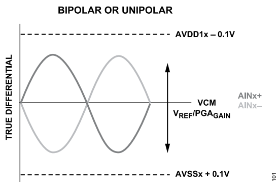
Figure 101. \Sigma - \Delta ADC Input Signal Configuration, True Differential
