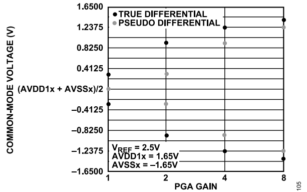
Figure 105. Maximum Common-Mode Voltage Range for a Maximum Differential Input Signal
