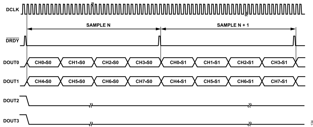
Figure 135. FORMAT0 = 0, FORMAT1 = 1—Channel 0 to Channel 3 Share DOUT0, and Channel 4 to Channel 7 Share DOUT1 (S0 Means Sample 0 and S1 Means Sample 1)
