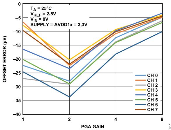
Figure 57. Offset Error vs. PGA Gain at 64 kSPS, High Resolution Mode
