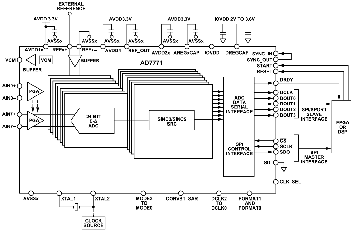
Figure 114. Pin Control Mode Connection Diagram with External Reference
