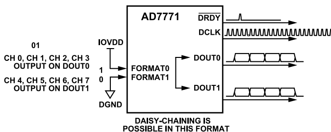
Figure 132. FORMATx Pin Configuration—FORMAT0 = 1, FORMAT1 = 0
