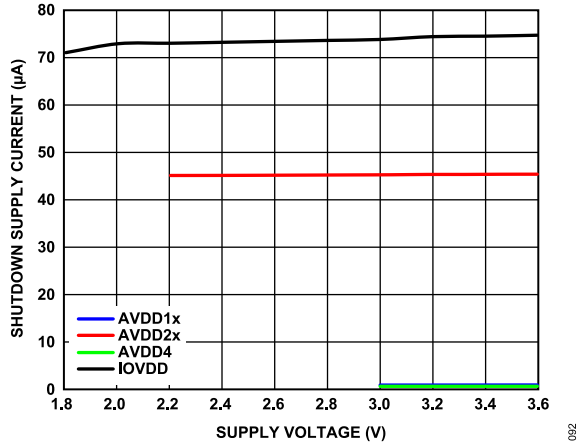
Figure 92. Shutdown Supply Current vs. Supply Voltage
