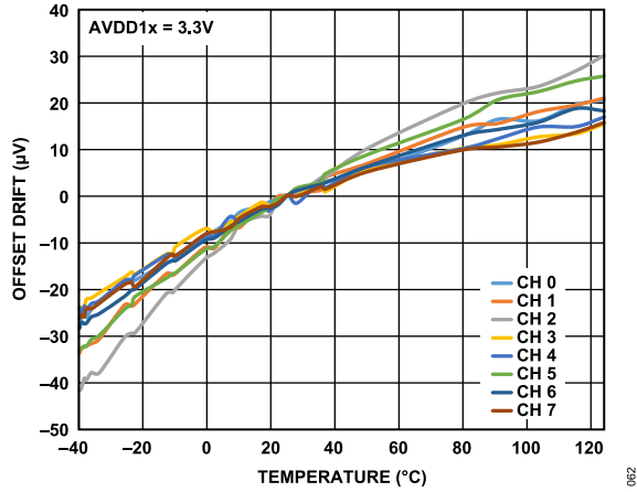
Figure 62. Offset Drift vs. Temperature
