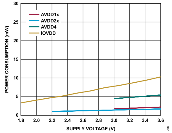
Figure 96. Power Consumption per Channel vs. Supply Voltage, Low Power Mode
