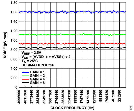
Figure 29. Noise vs. Clock Frequency, Low Power Mode
