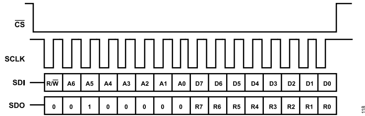
Figure 118. 16-Bit SPI Transfer—CRC Disabled
