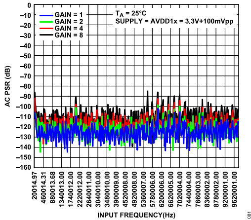
Figure 81. AC PSRR vs. Input Frequency at 128 kSPS, High Resolution Mode
