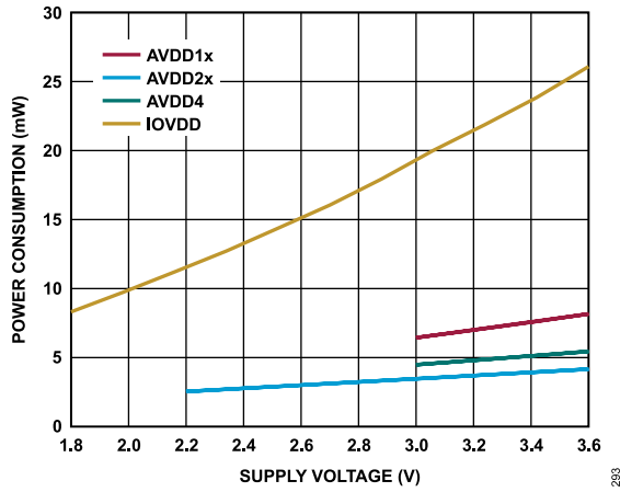
Figure 93. Power Consumption per Channel vs. Supply Voltage, High Resolution Mode
