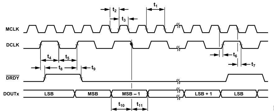
Figure 2. Data Interface Timing Diagram
