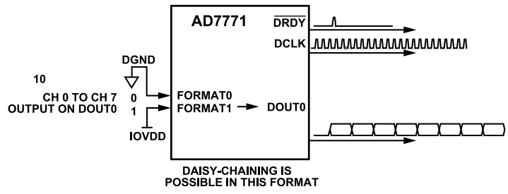
Figure 133. FORMATx Pin Configuration—FORMAT0 = 0, FORMAT1 = 1
