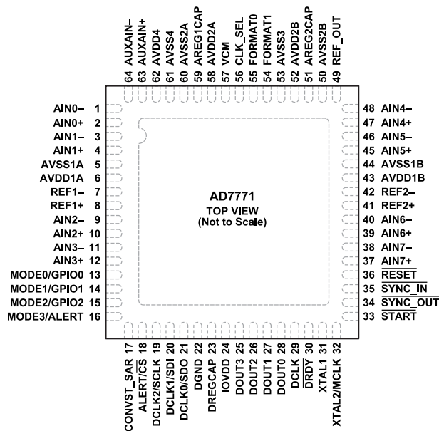
Figure 7. Pin Configuration
