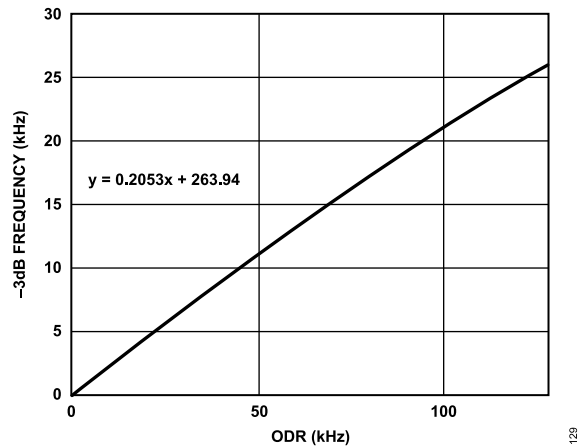
Figure 130. -3 dB Correction Factor, Sinc5 Filter Enabled
