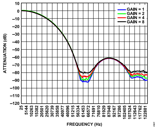
Figure 82. Filter Profiles at 64 kSPS, High Resolution Mode
