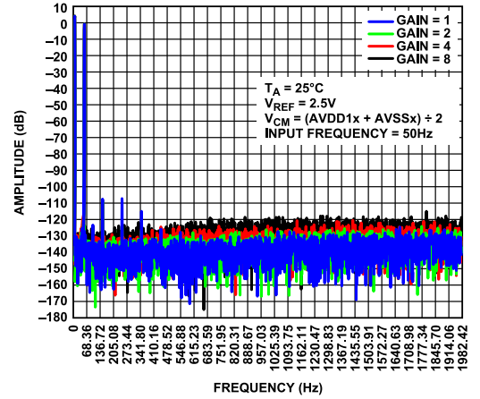
Figure 35. FFT Plot, Low Power Mode at 4 kSPS, Input Frequency ( f_{IN} ) = 50 Hz, Sinc3 Filter Enabled
