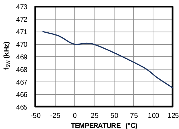
f_{SW} vs. Temperature R_{FREQ} = 62k\Omega
