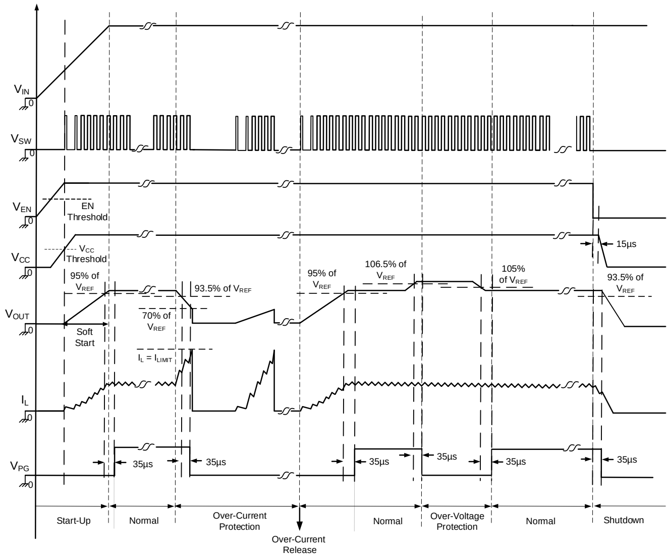
Figure 2: Timing Sequence
