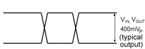
Figure 3. Single-Ended Swing
