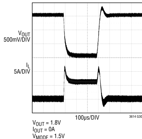
V_{OUT} Short to GND, Forced Continuous Mode
