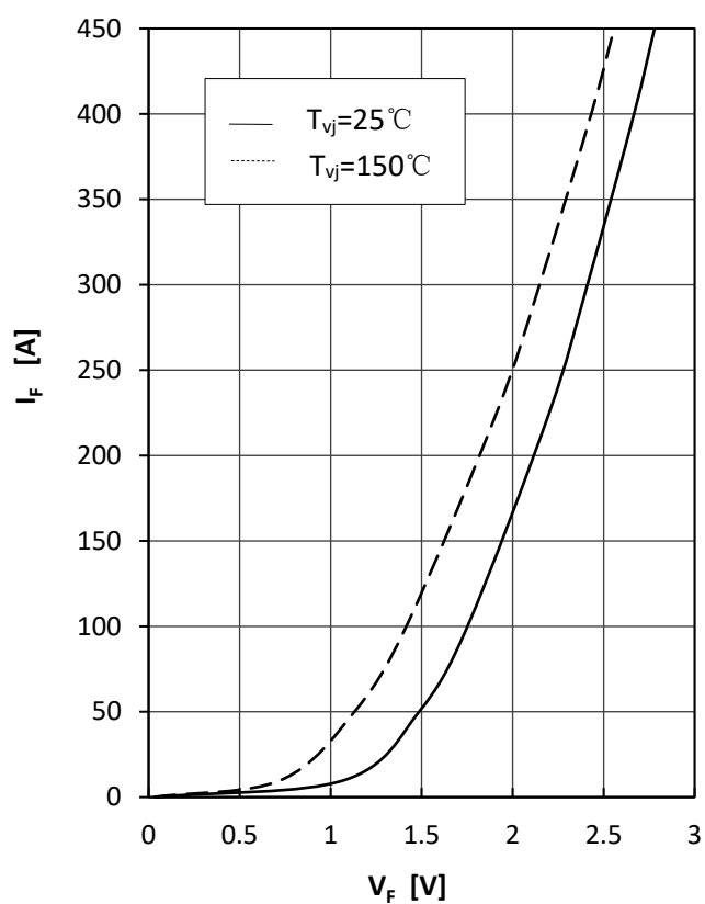
Fig7.Diode Foward Characteristics
