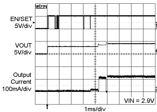
Figure 12. Power Up in 1.5x Mode
