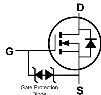
Equivalent Circuit
