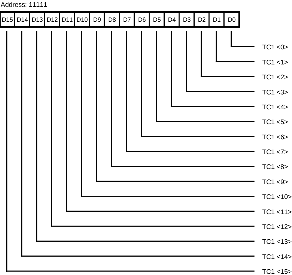
Figure 78. Time Constant 1 Register (TC1R)
