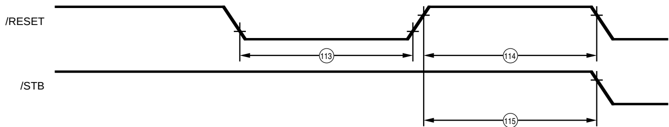
Figure 83. Reset Timing
