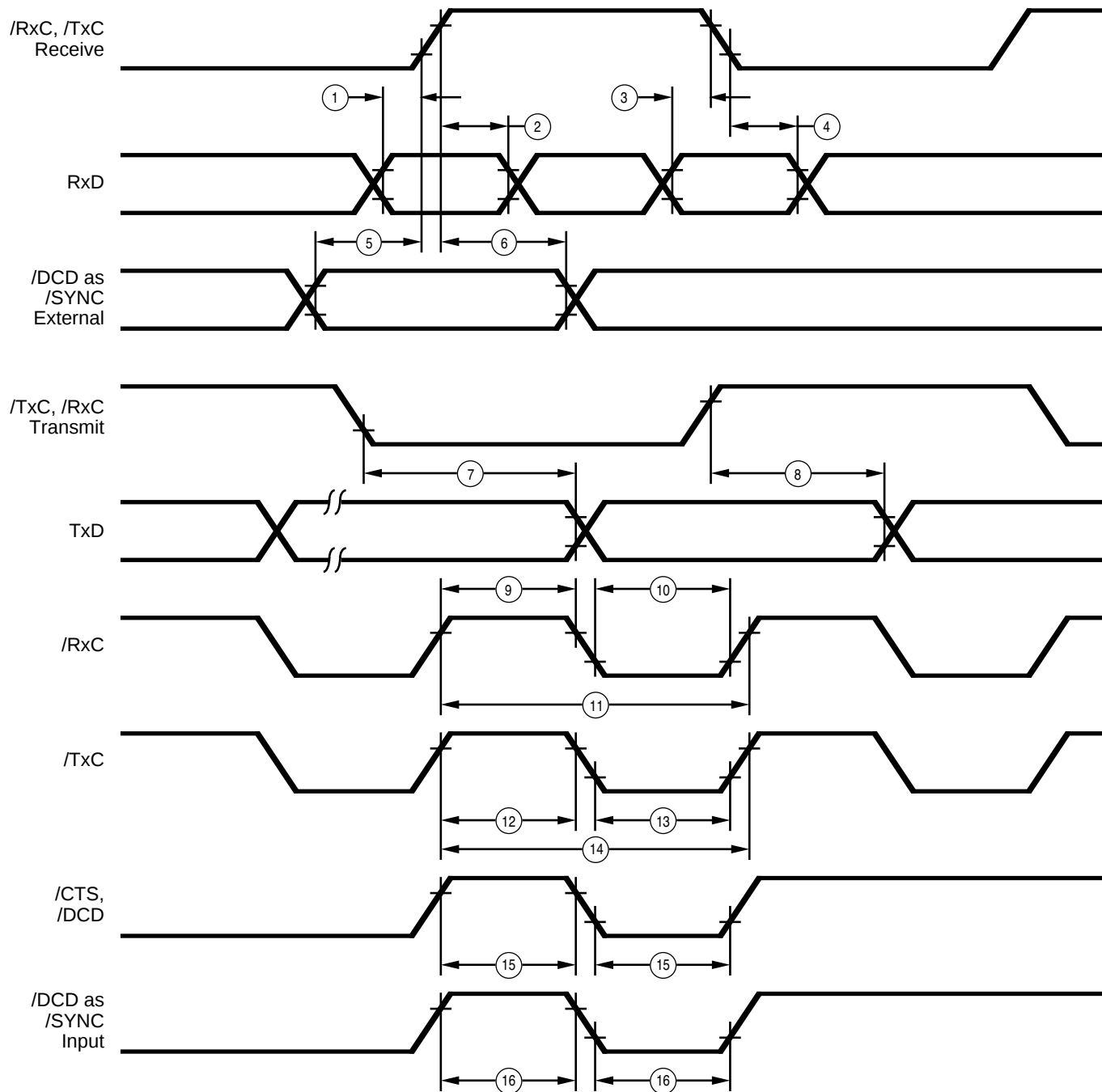
Figure 106. General Timing
