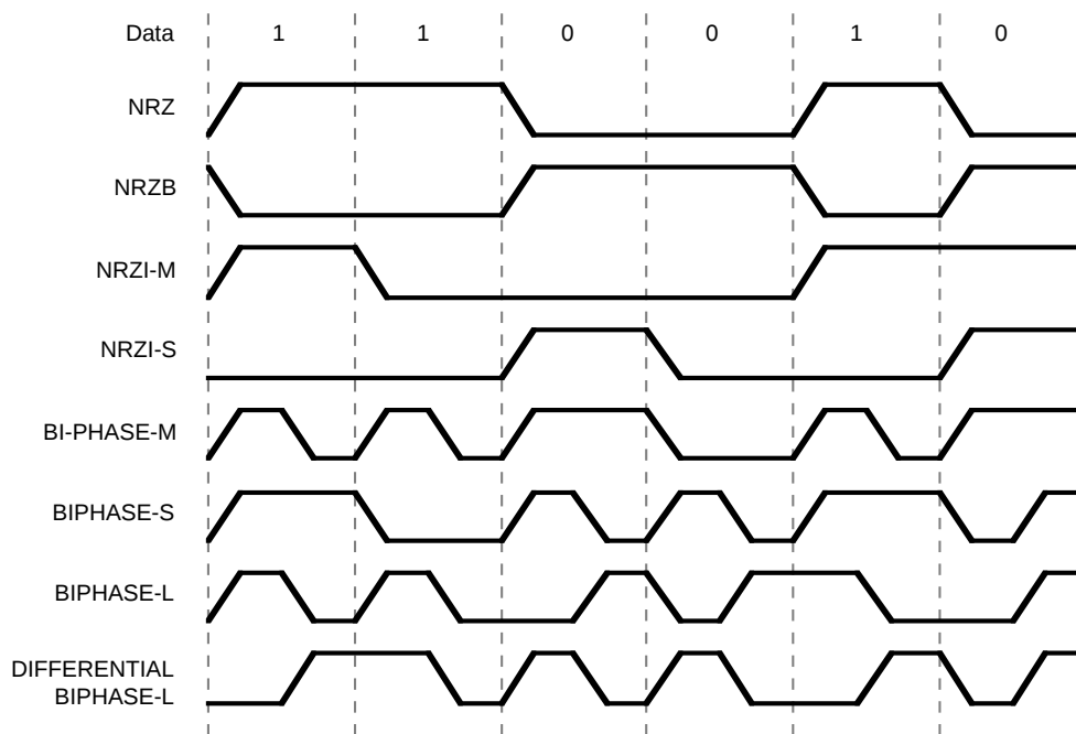
Figure 6. Data Encoding
