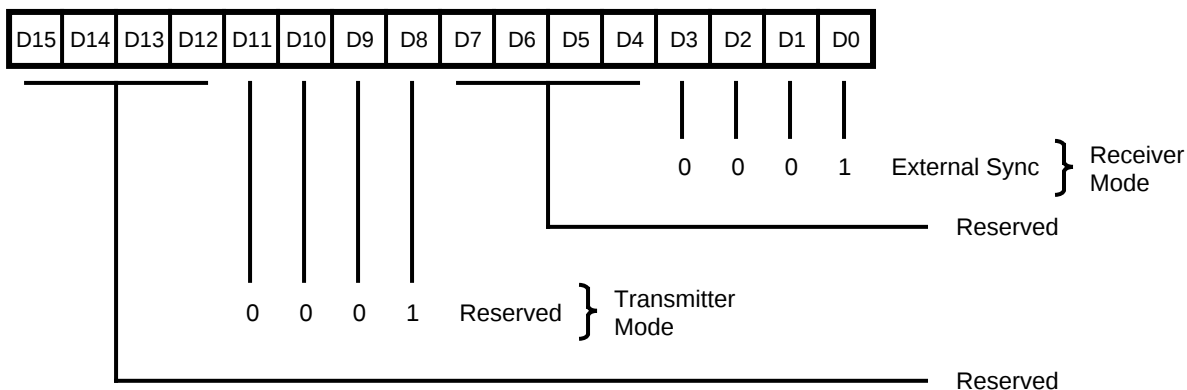
Figure 38. Channel Mode Register, External Sync Mode
