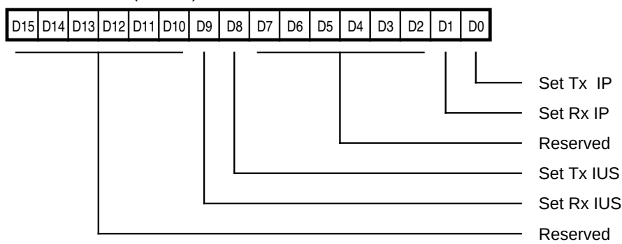
Figure 19. Set DMA Interrupt Register (SDIR)
