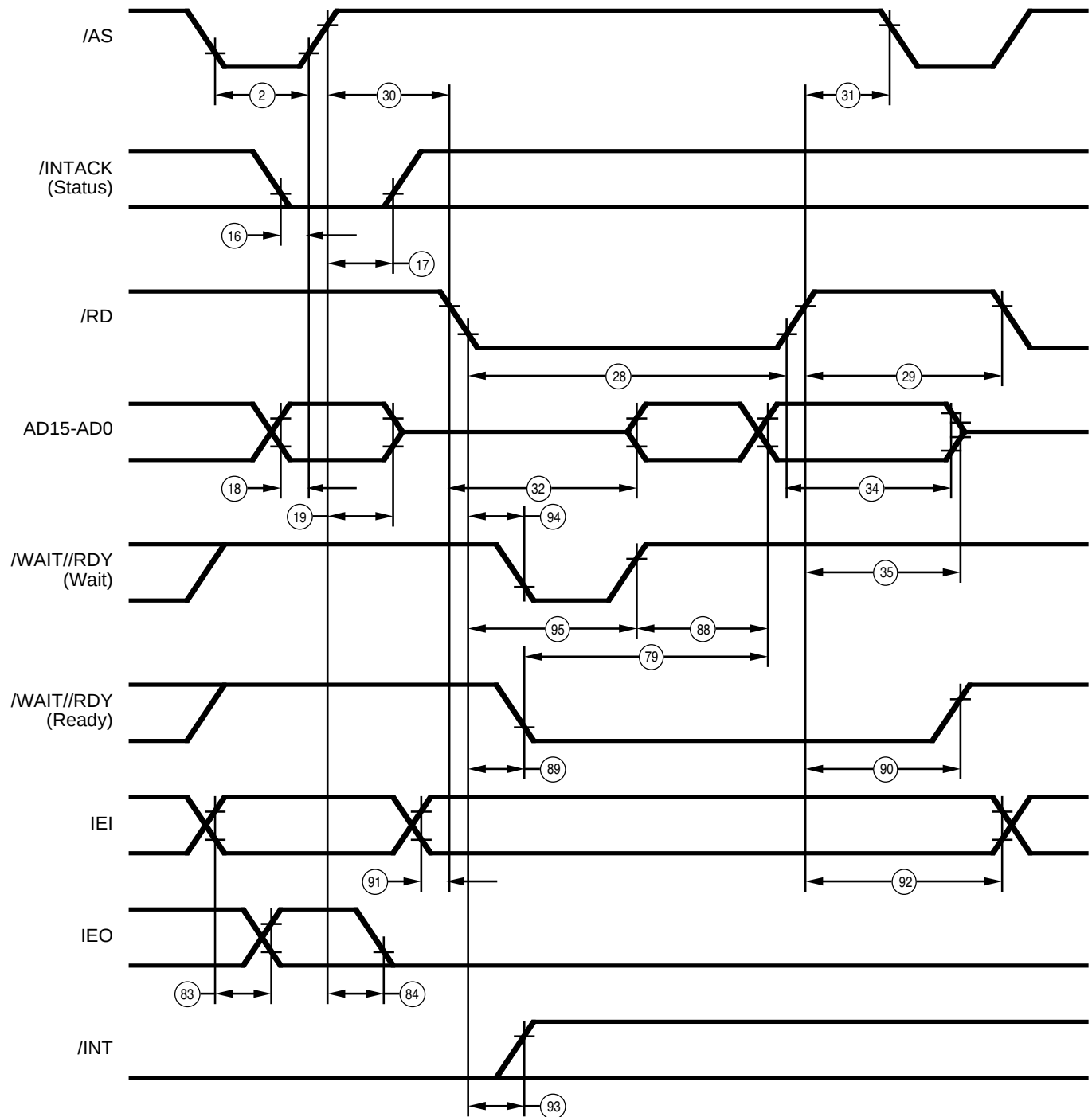
Figure 94. Multiplexed \overline{\text{RD}} Interrupt Acknowledge Cycle
