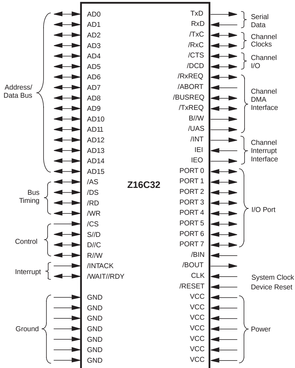
Figure 2. Z16C32 Pin Functions
