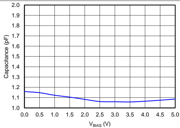
Figure 7. Capacitance vs V BIAS
