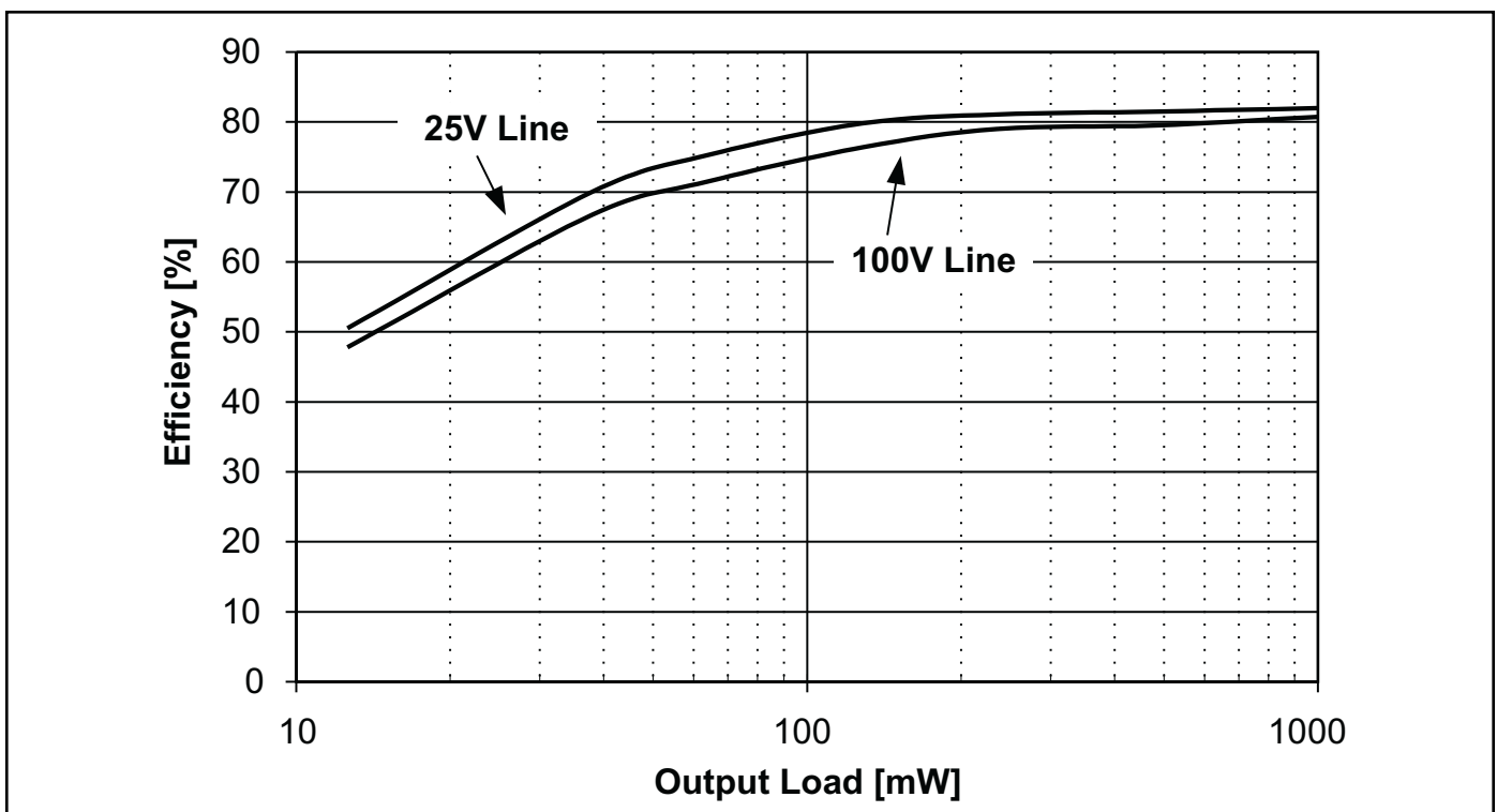
Figure 4. UCC3581 efficiency vs. line and load.
