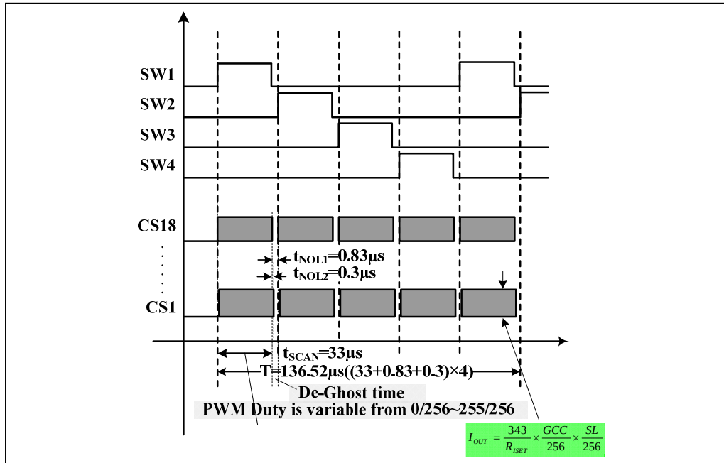
Figure 12 Scanning Timing
