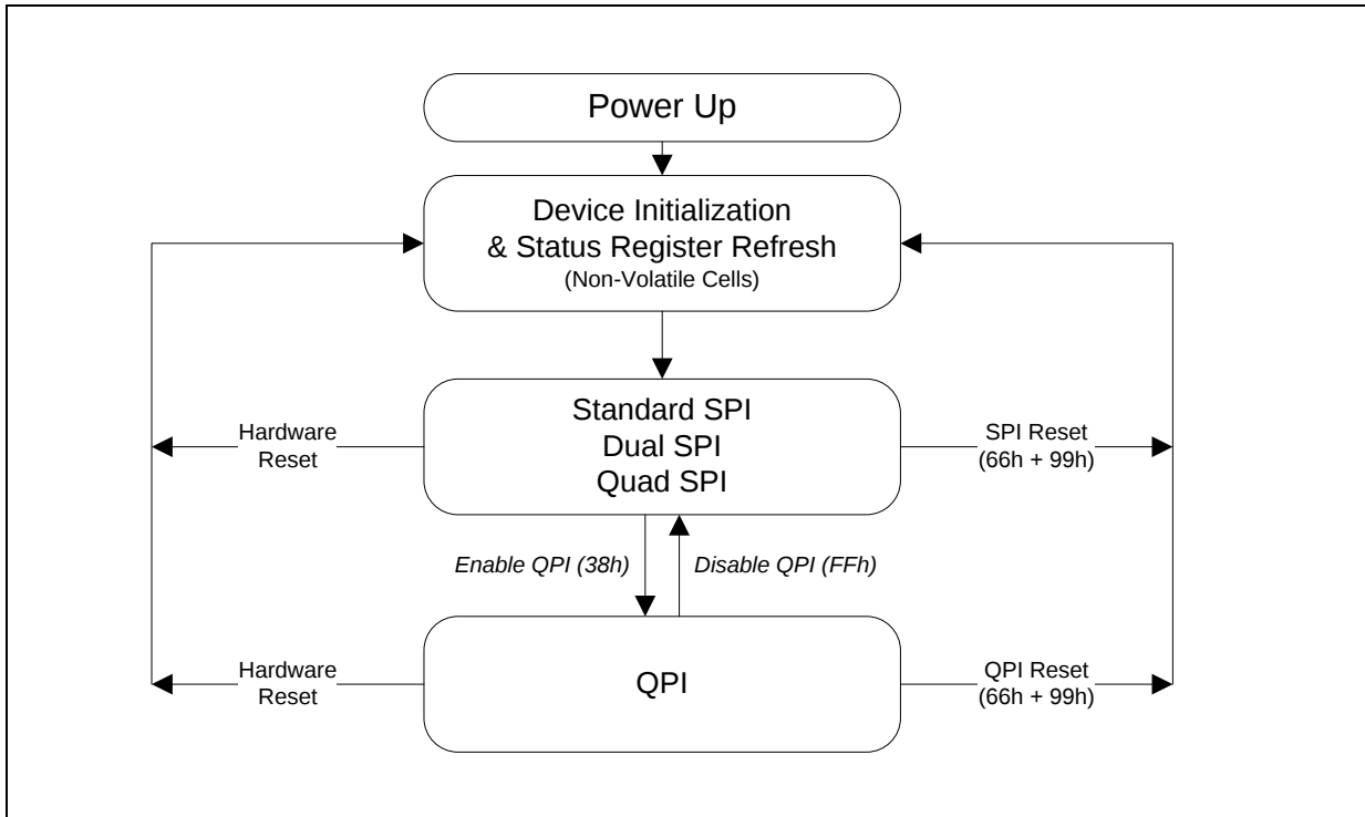
Figure 3. W25Q80RL Serial Flash Memory Operation Diagram
