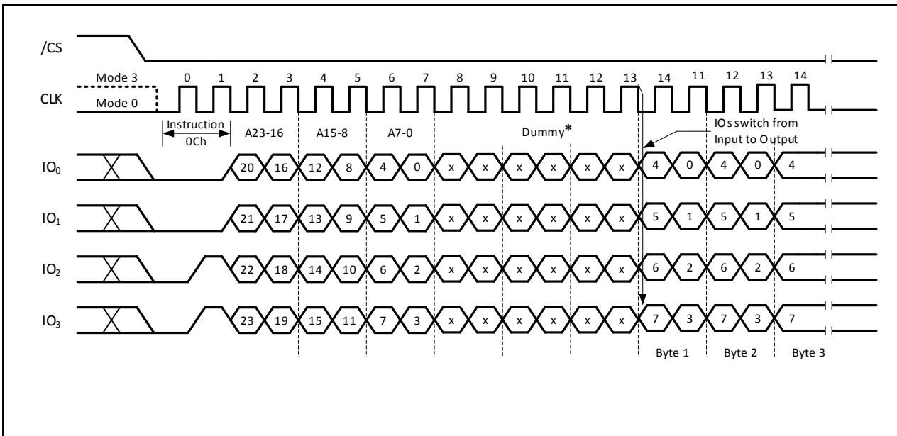
Figure 48. Burst Read with Wrap Instruction (QPI Mode only) "Set Read Parameters" instruction (C0h) can set the number of dummy clocks"
