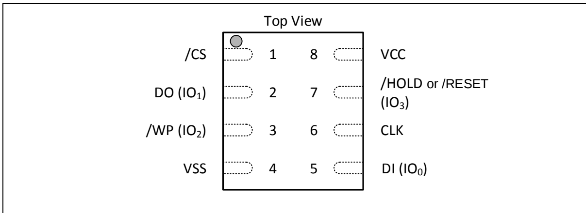
Figure 1b. Pad Assignments, XSON 2X3-mm (Package Code XH)
