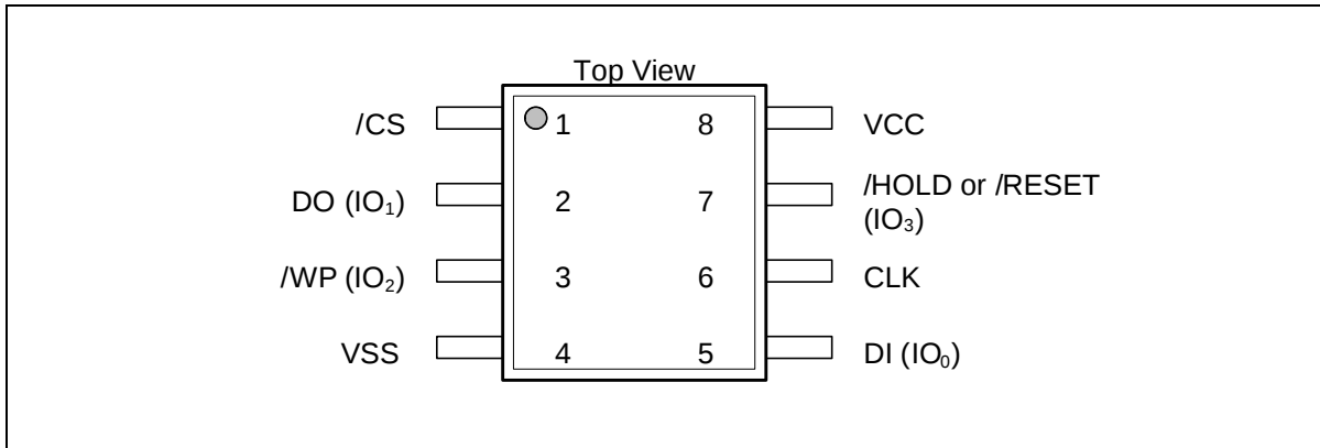
Figure 1a. Pin Assignments, 8-pin SOIC 150/208-MIL (Package Code SN, SS)
