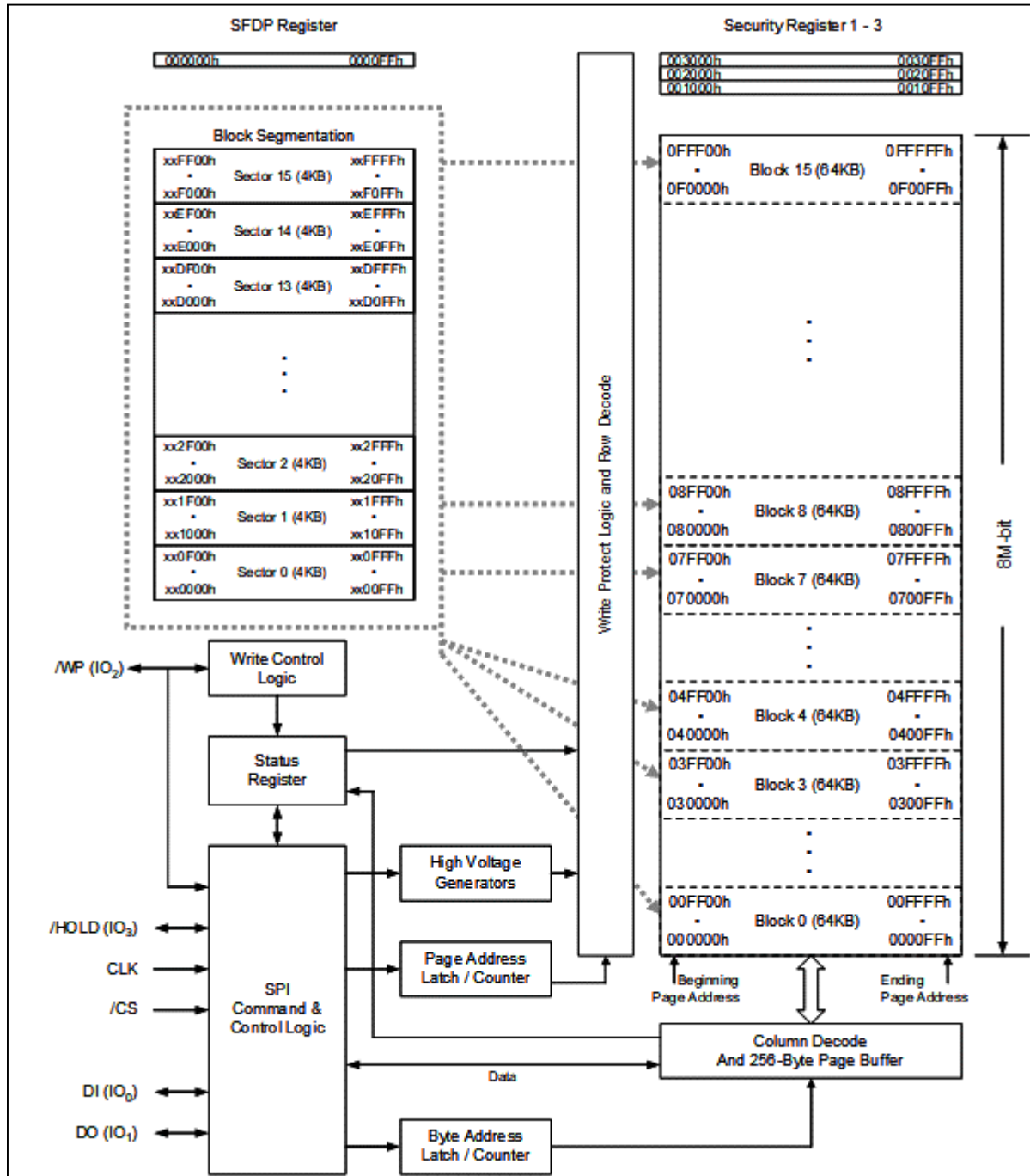
Figure 2. W25Q80RL Serial Flash Memory Block Diagram
