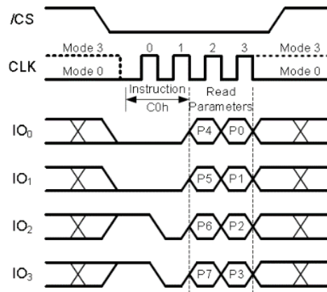
Figure 54. Set Read Parameters Instruction (QPI Mode) "Set Read Parameters" instruction (C0h) can set the number of dummy clocks"
