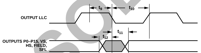
Figure 3. Pixel Port and Control Output Timing
