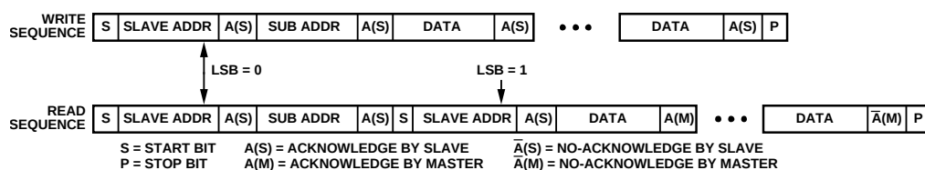
Figure 39. Read and Write Sequence
