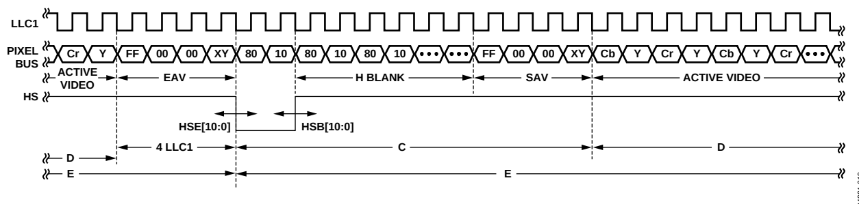
Figure 19. HS Timing
