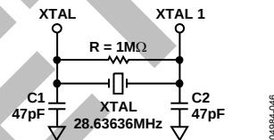
Figure 43. Crystal Circuit
