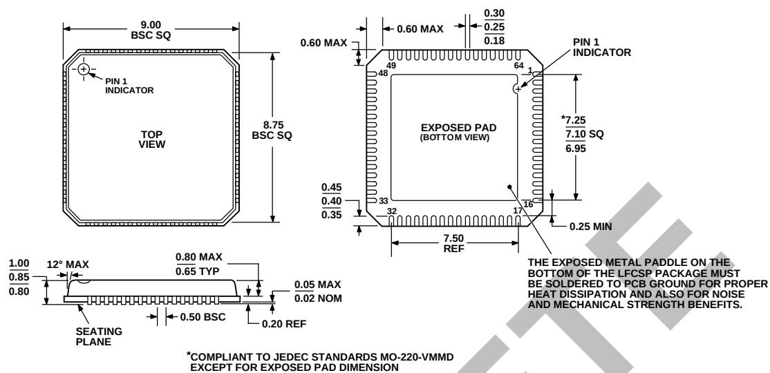
Figure 46. 64-Lead Lead Frame Chip Scale Package [LFCSP_VQ] 9 × 9 mm Body, Very Thin Quad (CP-64-3) Dimensions shown in millimeters
