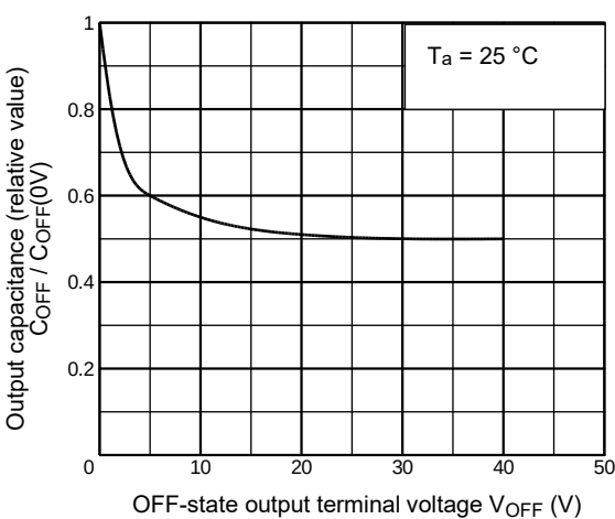
Fig.12.10 C_{OFF} / C_{OFF(0V)} - V_{OFF}
