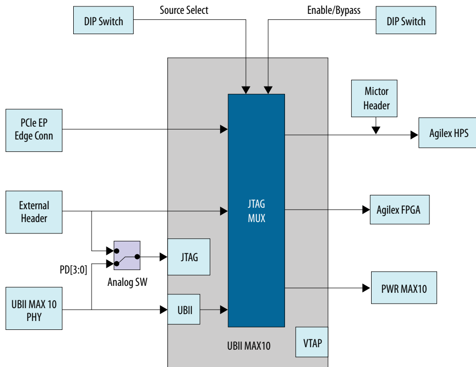
Figure 13. JTAG chain on the Development Kit
