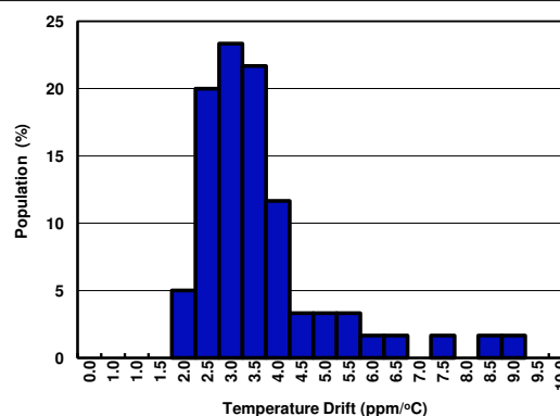
Figure 7-4. Internal Reference Temperature Drift Histogram
