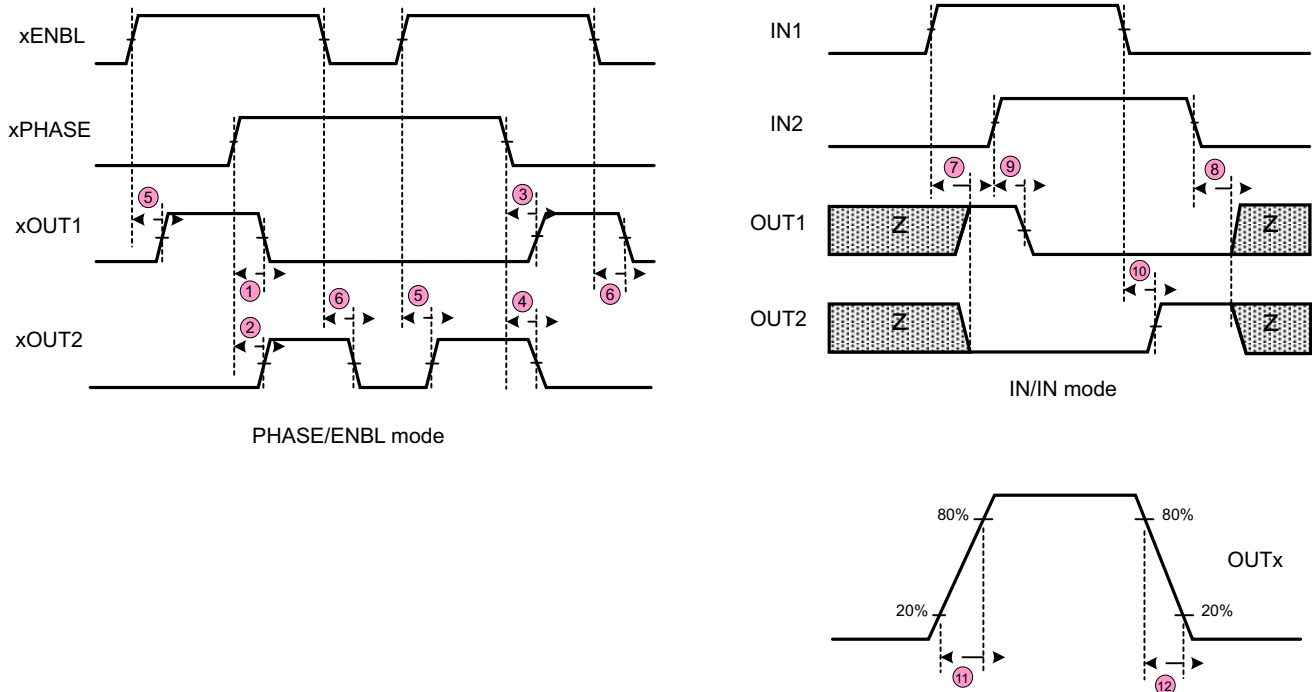
Figure 1. Timing Requirements
