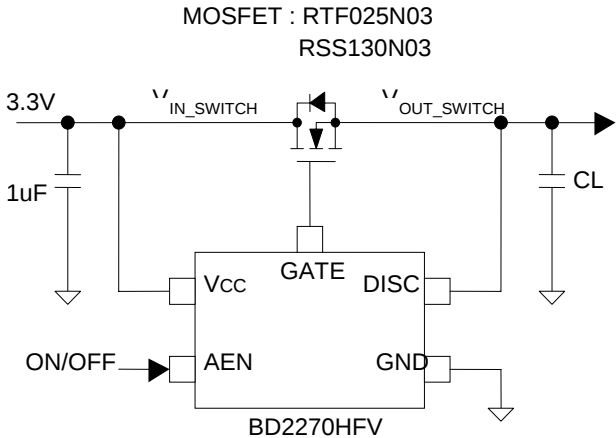
Figure 29. Switch Rise / Fall Characteristics Measurement Circuit Diagram
