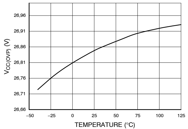
Figure 8. V_{CC(ovp)} vs. Temperature
