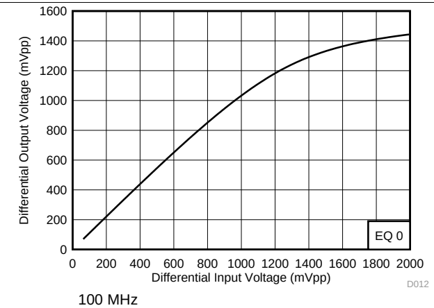
Figure 18. Upstream-to-Downstream Linearity Performance at 100 MHz
