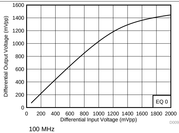
Figure 15. Downstream-to-Upstream Linearity Performance at 100 MHz
