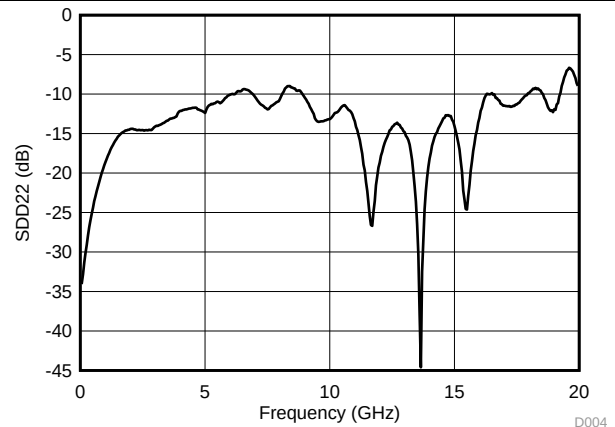
Figure 10. Output Return Loss Performance of the Downstream Ports
