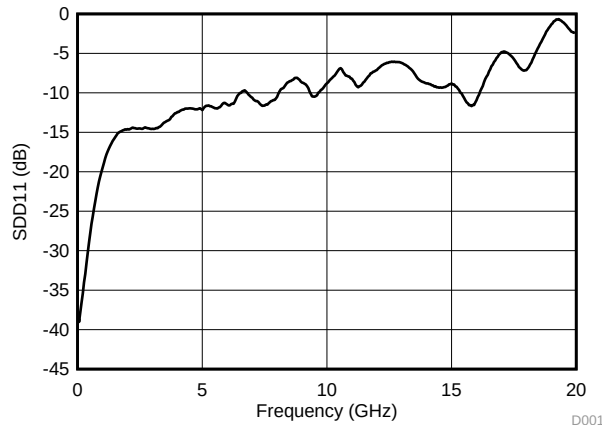
Figure 9. Input Return Loss Performance of the Downstream Ports
