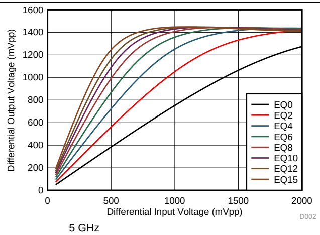
Figure 16. Upstream-to-Downstream Linearity Performance at 5 GHz
