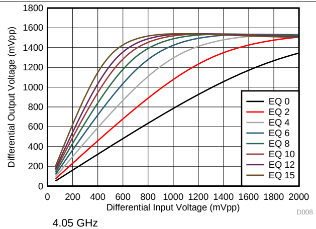
Figure 14. Downstream-to-Upstream Linearity Performance at 4.05 GHz
