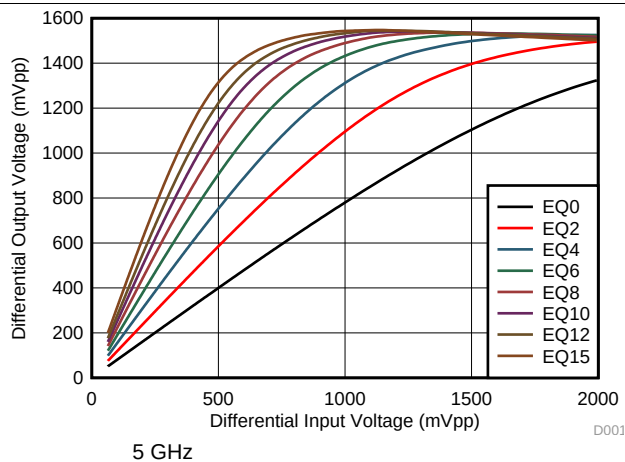
Figure 13. Downstream-to-Upstream Linearity Performance at 5 GHz
