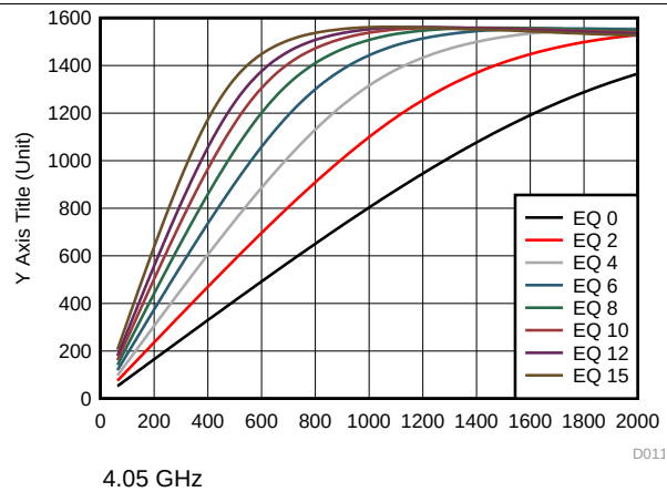
Figure 17. Upstream-to-Downstream Linearity Performance at 4.05 GHz
